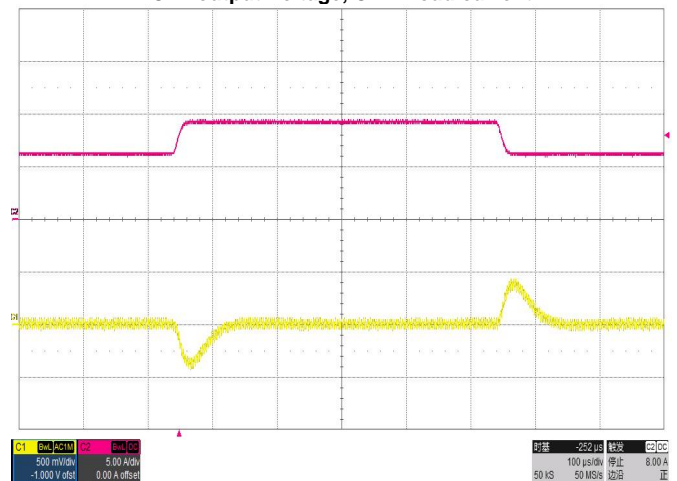
Transient Response V_{IN}=36V , Step from 50%-75%-50% C1-- output Voltage, C2 -- Load current
