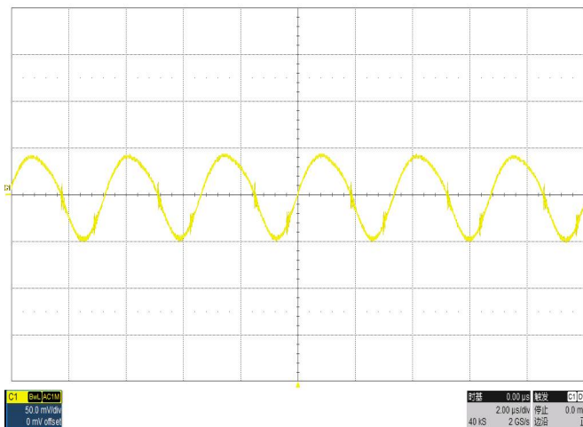
Noise V_{IN}=36V , I_O=12.5A , 20MHz Bandwidth
