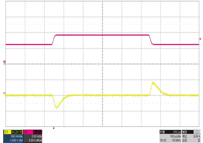
Transient Response V_{IN}=18V , Step from 50%-75%-50% C1-- output Voltage, C2 -- Load current
