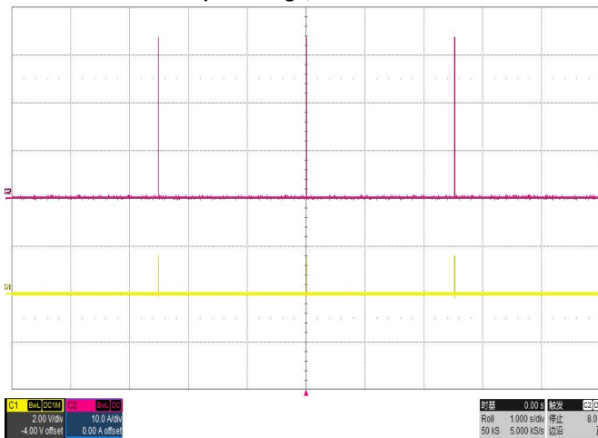
Short-Circuit Output VIN=24V C1-- output Voltage, C2 -- Load current
