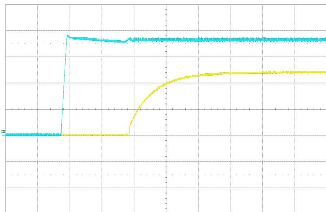
Start-up V_{IN}=24V , I_O=12.5A C1-- output Voltage, C3 -- input Voltage
