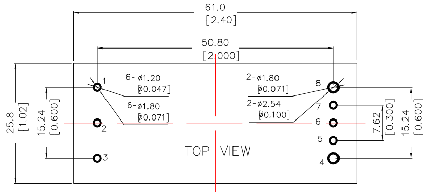
Component side footprint
