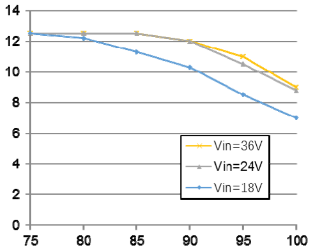
Ambient Temperature vs. Load Current 铝板尺寸: 270mm*165mm*10mm
