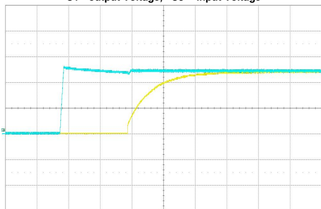
Start-up V_{IN}=18V , I_O=12.5A C1-- output Voltage, C3 -- input Voltage
