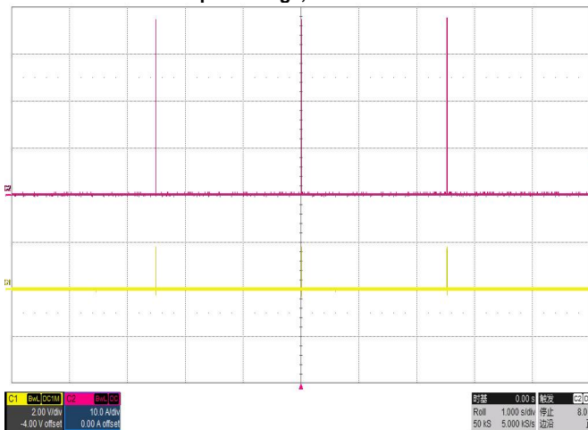
Short-Circuit Output VIN=36V C1-- output Voltage, C2 -- Load current
