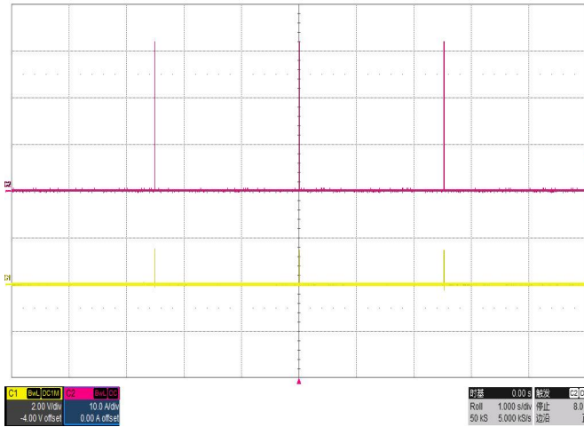
Short-Circuit Output VIN=18V C1-- output Voltage, C2 -- Load current
