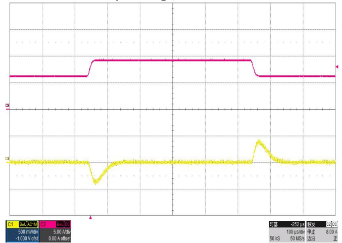
Transient Response V_{IN}=24V , Step from 50%-75%-50% C1-- output Voltage, C2 -- Load current
