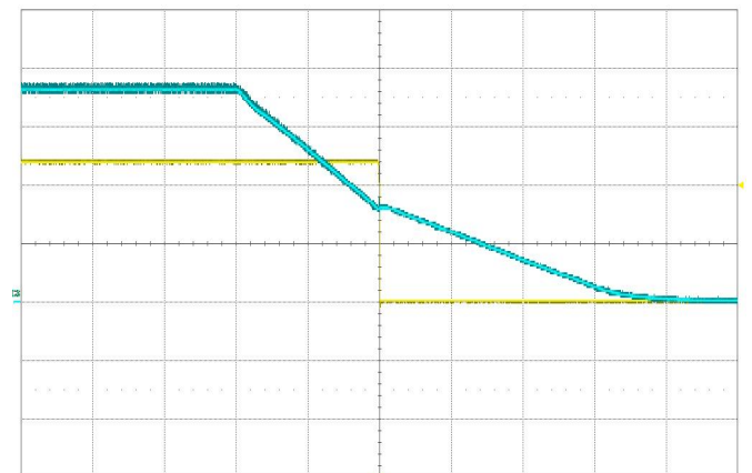
Shut-down V_{IN}=24V , I_O=12.5A C1-- output Voltage, C3 -- input Voltage
