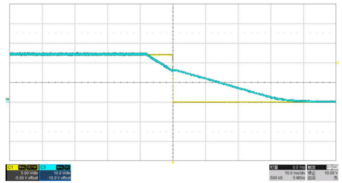
Shut-down V_{IN}=24V , I_O=12.5A C1-- output Voltage, C3 -- input Voltage
