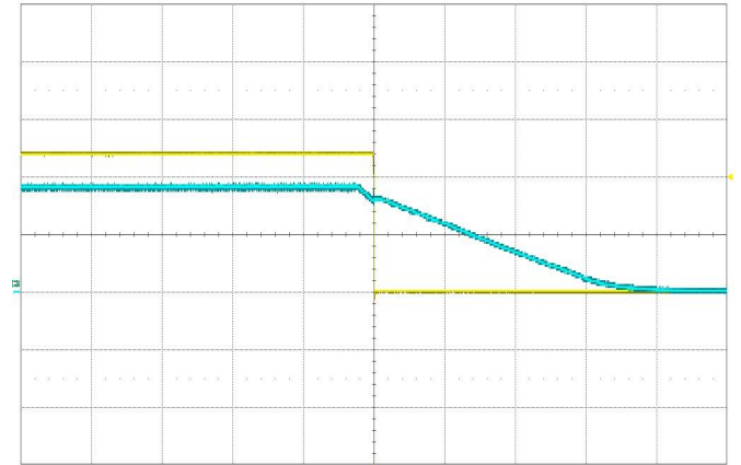
Shut-down V_{IN}=18V , I_O=12.5A C1-- output Voltage, C3 -- input Voltage
