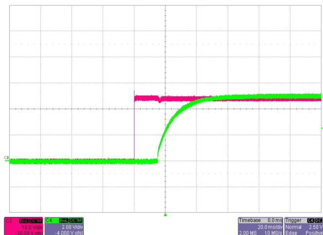
Start-up V_{IN}=24V , I_O=24A C4-- output Voltage, C2 -- input Voltage
