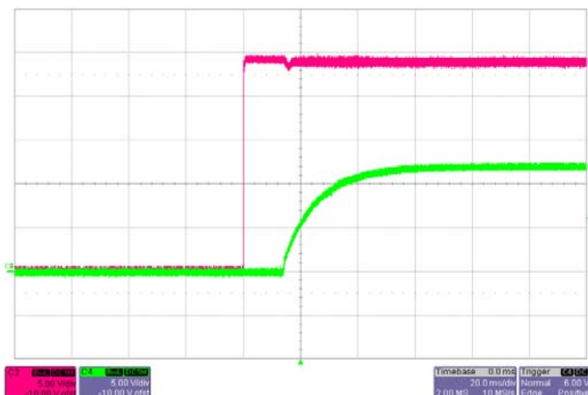
Start-up V_{IN}=24V , I_O=10A C4-- output Voltage, C2 -- input Voltage
