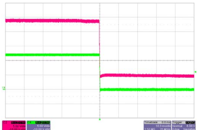
Shut-down V_{IN}=24V , I_O=10A C4-- output Voltage, C2 -- input Voltage
