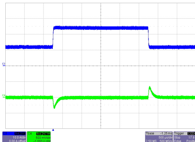
Transient Response V_{IN}=24V , Step from Half-Full- Half C1-- output Voltage, C3 -- Load current
