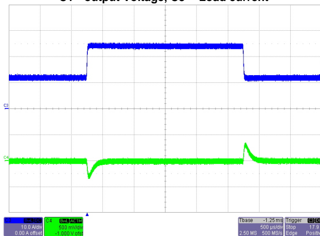
Transient Response V_{IN}=48V , Step from Half-Full- Half- C4-- output Voltage, C3 -- Load current
