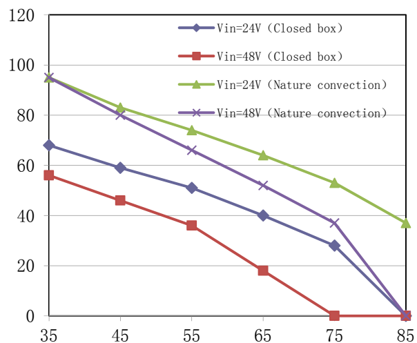
Ambient Temperature vs. Load Current (Vin=24V/48V) Inside the box size: 185mm*185mm*130mm
