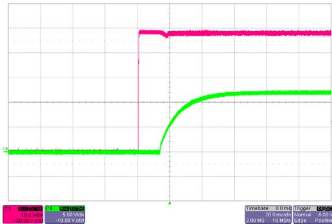
Start-up V_{IN}=48V , I_O=10A C4-- output Voltage, C2 -- input Voltage
