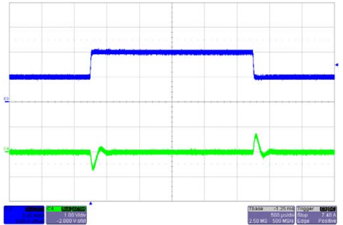
Transient Response V_{IN}=24V , Step from Half-Full- Half C1-- output Voltage, C3 -- Load current
