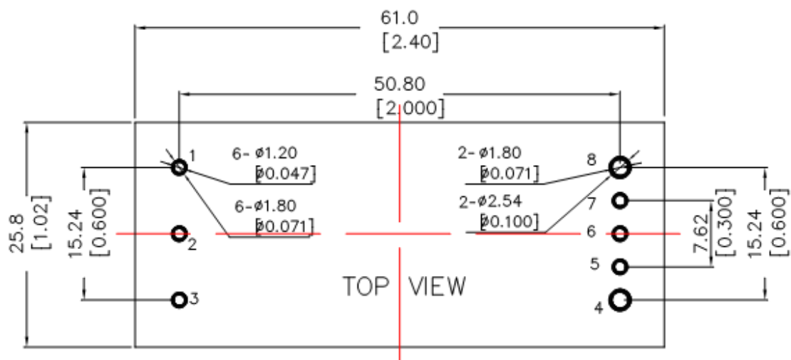
Component side footprint
