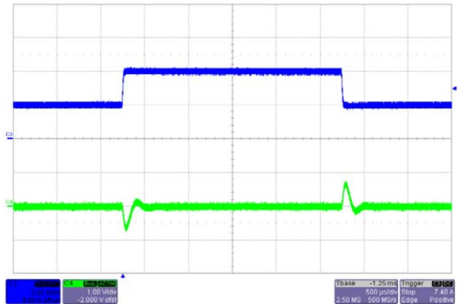
Transient Response V_{IN}=48V , Step from Half-Full- Half C4-- output Voltage, C3 -- Load current
