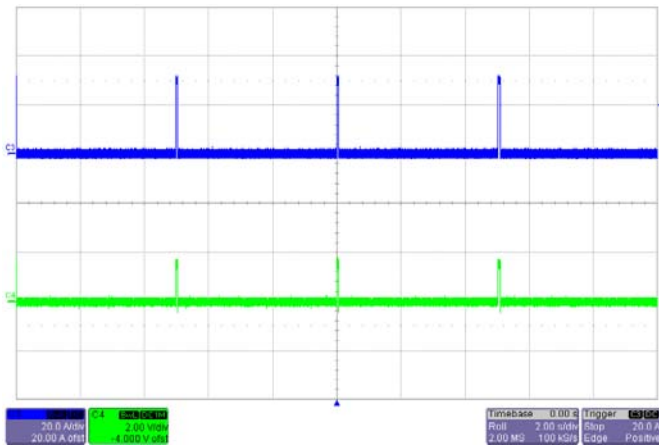
Short-Circuit Output V_{IN}=24V C4-- output Voltage, C3 -- Load current
