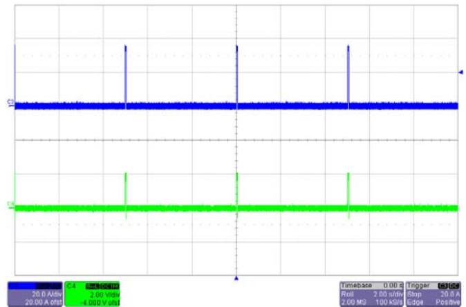
Short-Circuit Output V_{IN}=48V C4-- output Voltage, C3 -- Load current
