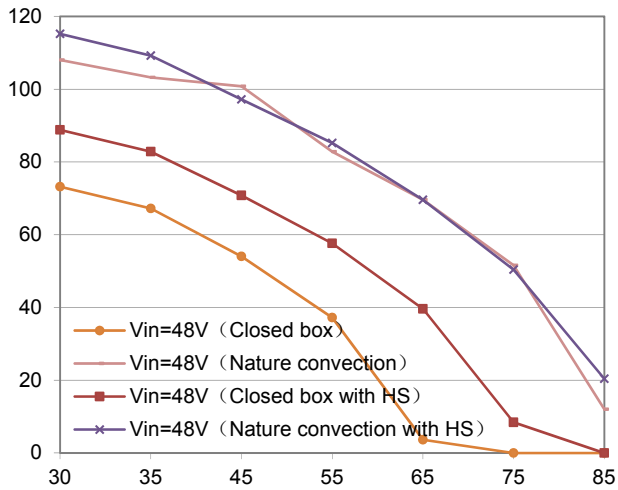
Ambient Temperature vs. Load Current (Vin=48V) Inside the box size: 185mm*185mm*130mm
