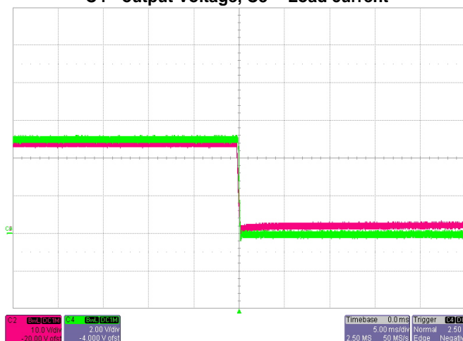
Shut-down V_{IN}=24V , I_O=24A C4-- output Voltage, C2 -- input Voltage
