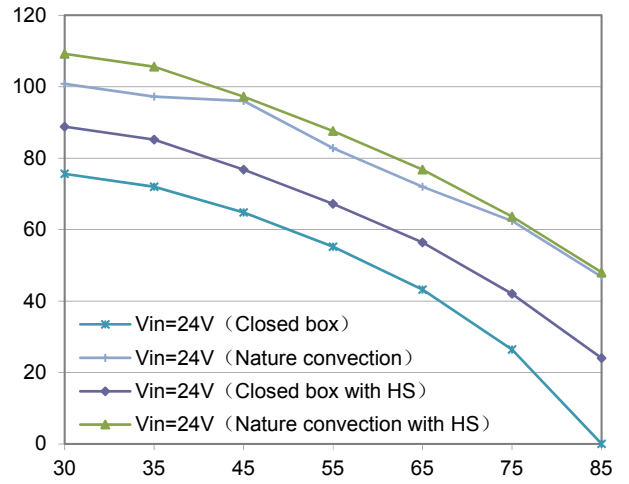
Ambient Temperature vs. Load Current (Vin=24V) Inside the box size: 185mm*185mm*130mm
