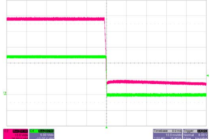
Shut-down V_{IN}=48V , I_O=10A C4-- output Voltage, C2 -- input Voltage
