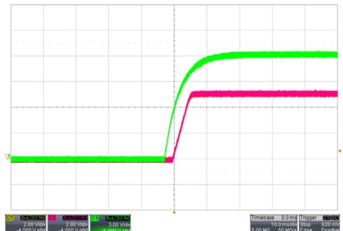
Start-up With VIN=12V, IO=3A
