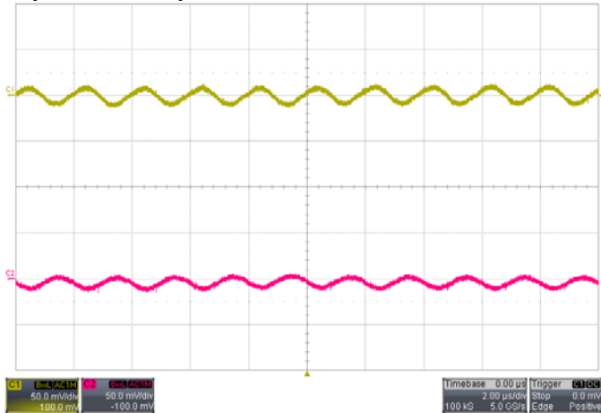
Ripple&Noise VIN=5V, IO=3A for both channel C1: Vo1; C4: Vo2
