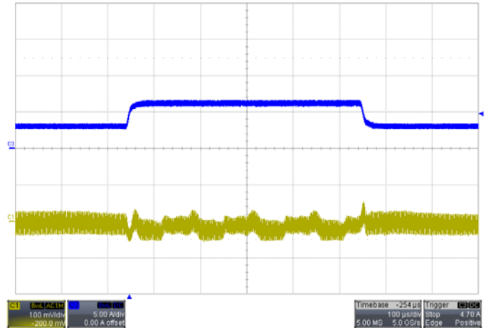
Transient Response VIN=12V, IO=3A Step from 1.5A~3A~1.5A(Vo1)
