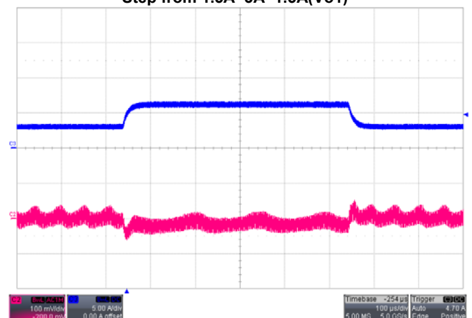
Transient Response VIN=12V, IO=3A Step from 1.5A~3A~1.5A(Vo2)
