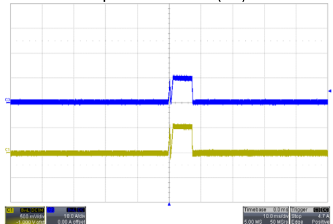
Short-Circuit Output VIN=12V(Vo1)
