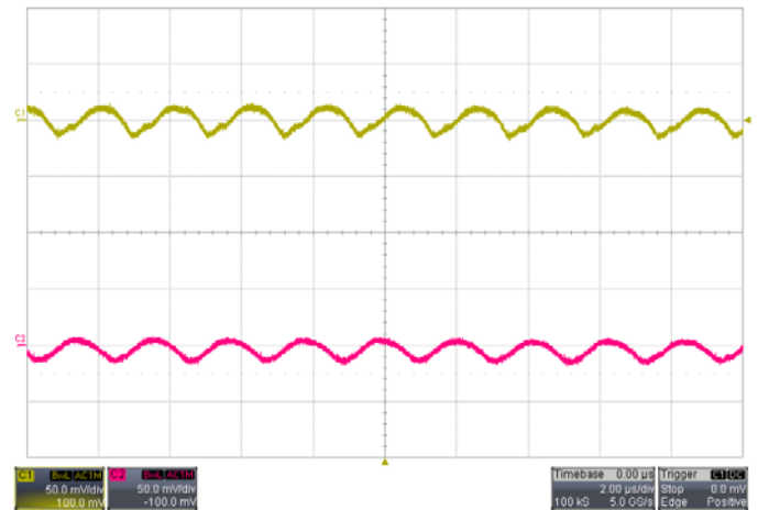
Ripple&Noise VIN=12V, IO=3A for both channel C1: Vo1; C4: Vo2
