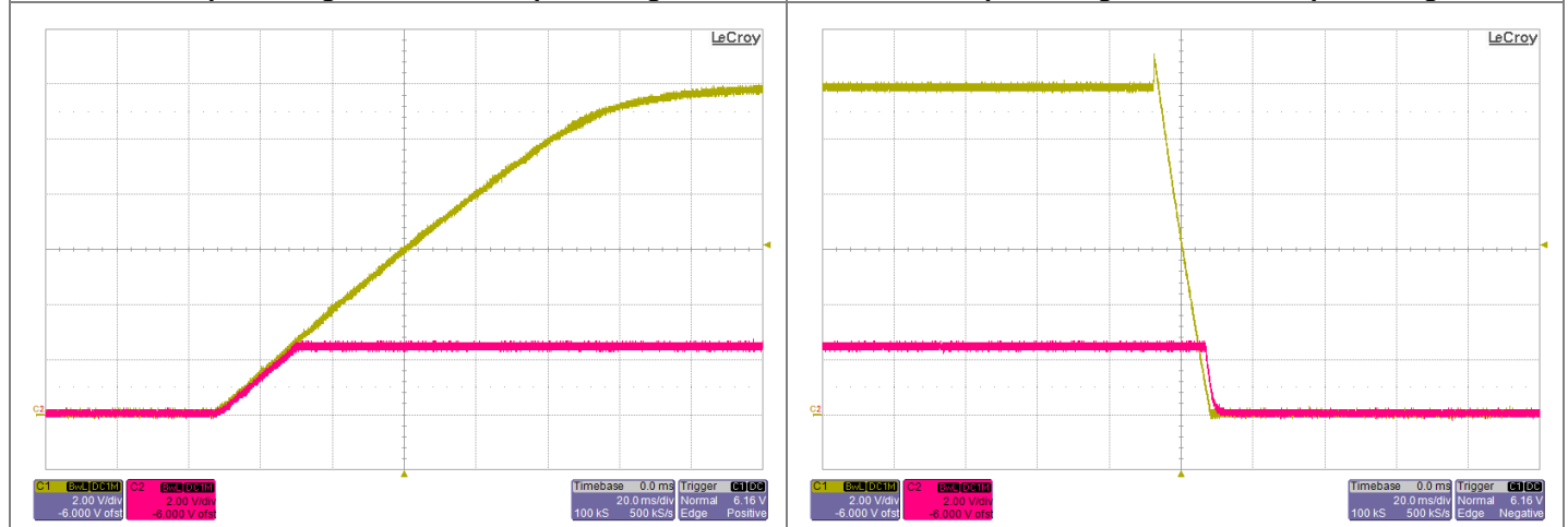
Power Down with Auto-Track Control V_{Track}=5.0V , I_O=8A Red: EasyTrack™ Control Voltage Yellow: Output Voltage
