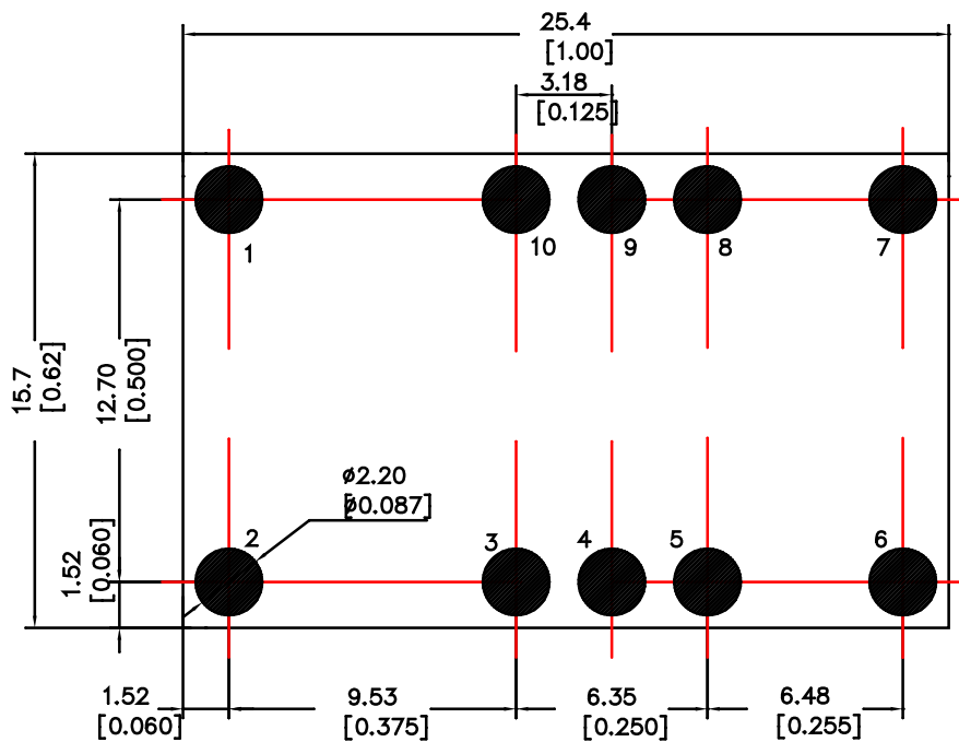
Component-side footprint
