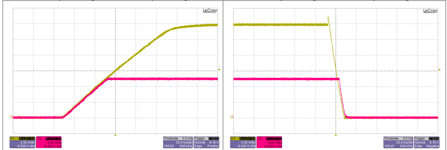
Power Up with Auto-Track Control V_{Track}=5.0V , I_O=8A Red: EasyTrack™ Control Voltage Yellow: Output Voltage
