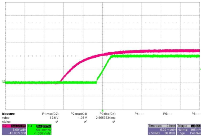
Start-up V_{IN}=12V , I_O=8A Red: Input Voltage Yellow: Output Voltage
