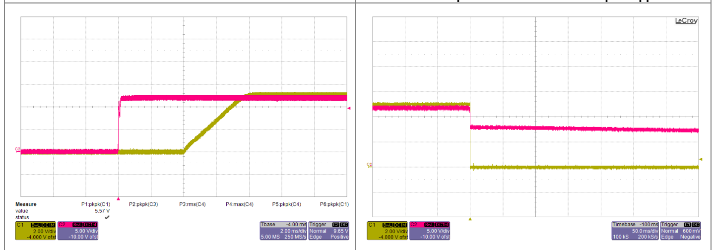
Start-up V_{IN}=12V , I_O=8A Red: Input Voltage Yellow: Output Voltage
