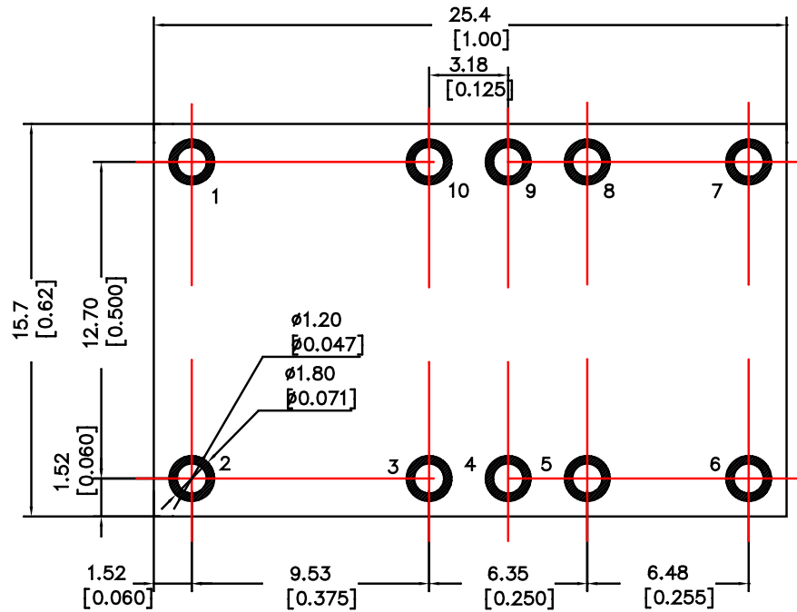
Component-side footprint
