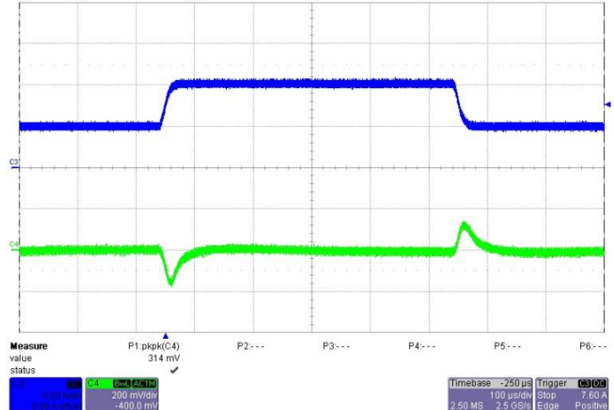
Transient Response V_{IN}=12V , Step from 4A-8A-4A Blue: Output Current Yellow: Output Ripple
