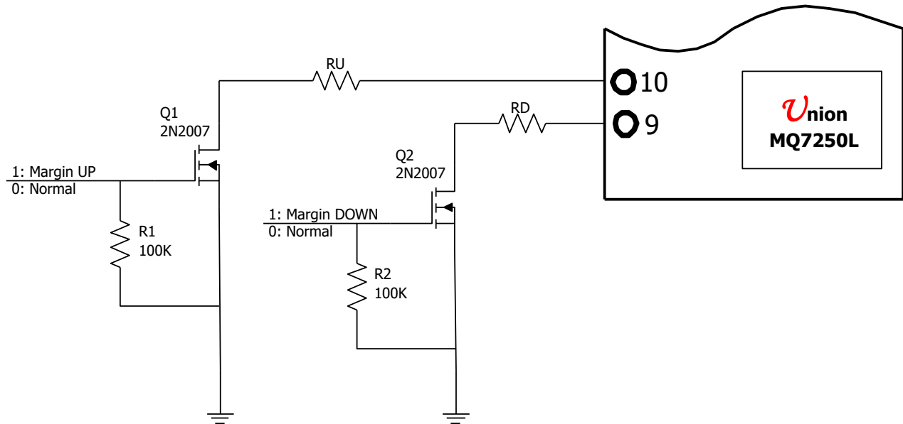
Fig4 Margin up and Margin down application circuit
