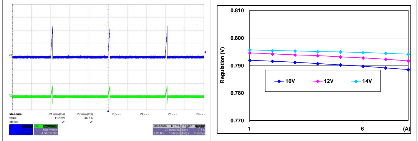
Regulation Output voltage vs. Load Current
