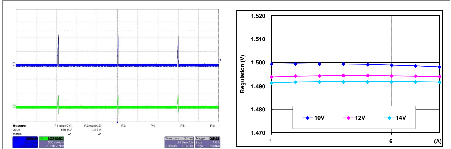
Regulation Output voltage vs. Load Current
