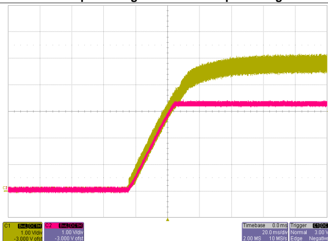
Power Up with EasyTrack™ Control V_{Track}=5.0V , I_O=30A Yellow: EasyTrack™ Control Voltage Red: Output Voltage
