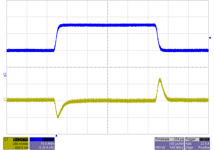
Transient Response V_{IN}=5.0V , Step from 15A~30A~15A Blue: Output Current Yellow: Output Ripple
