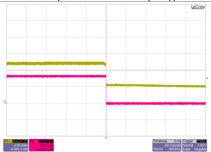
Shut-down V_{IN}=5.0V , I_O=30A Red: Input Voltage Yellow: Output Voltage
