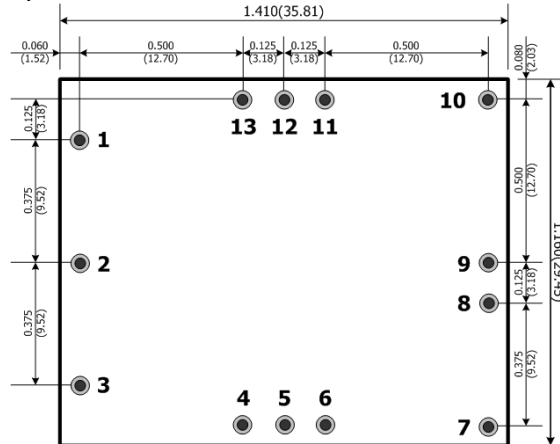
Component-side footprint
