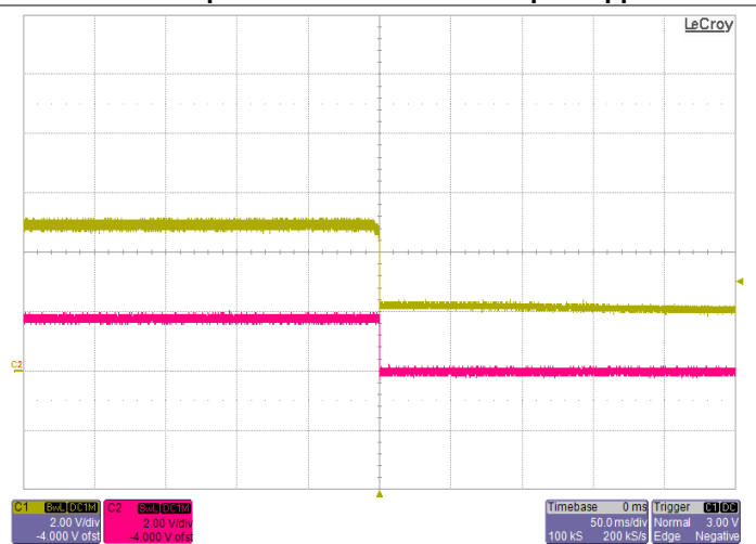
Shut-down V_{IN}=5.0V , I_O=30A Red: Input Voltage Yellow: Output Voltage
