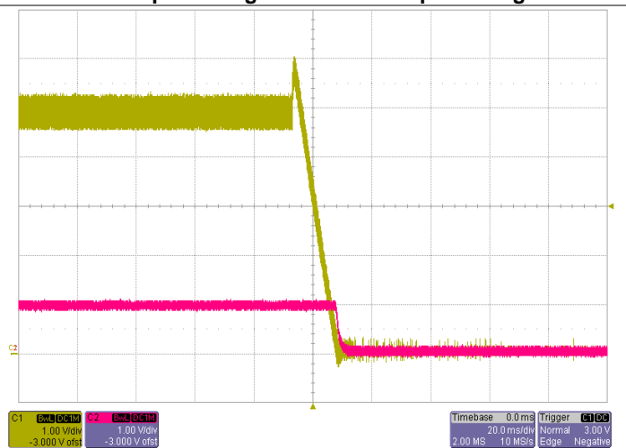
Power Down with EasyTrack™ Control V_{Track}=5.0V , I_O=30A Yellow: EasyTrack™ Control Voltage Red: Output Voltage
