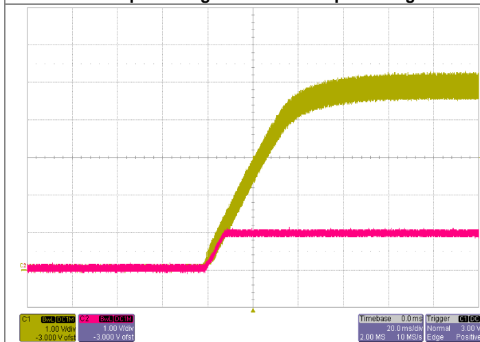
Power Up with EasyTrack™ Control V_{Track}=5.0V , I_O=30A Yellow: EasyTrack™ Control Voltage Red: Output Voltage
