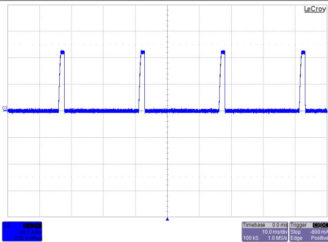
Short-Circuit Output V_{IN}=5.0V
