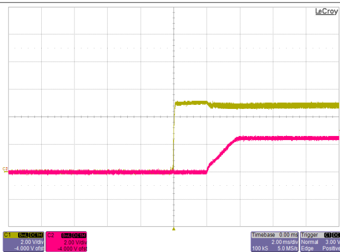
Start-up V_{IN}=5.0V , I_O=30A Red: Input Voltage Yellow: Output Voltage
