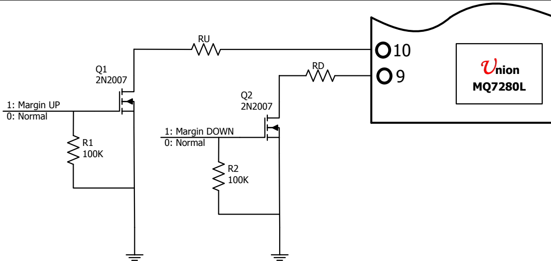
Fig4 Margin up and Margin down application circuit
