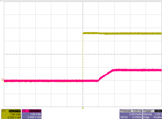
Power Up with ON/OFF Control Yellow: ON/OFF Control Voltage Red: Output Voltage
