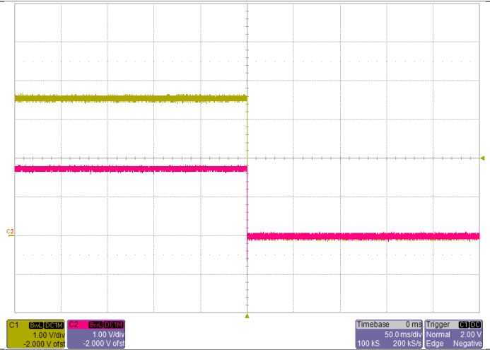
Power Down with ON/OFF Control Yellow: ON/OFF Control Voltage Red: Output Voltage
