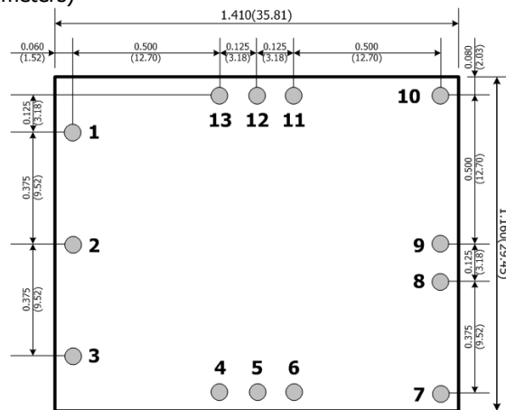
Component-side footprint
