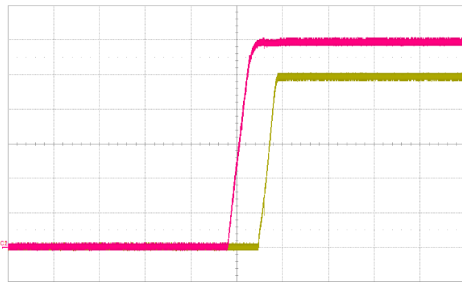
Measure value status P1:pkpk(C1) 5.15 V C1: 1.00 V/div, -3.000 V ofst C2: 2.00 V/div, -6.000 V ofst Timebase: 0.0 ms, Trigger: 10.0 ms, Normal, 5.00 V, 2.50 MS, 25 MS/s, Edge, Positive
