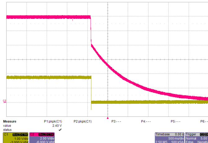
Shut-down V_{IN}=12V , I_O=26A Red: Input Voltage Yellow: Output Voltage
