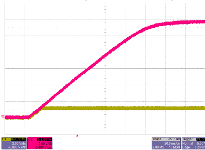
Power Up with EasyTrack™ Control V_{Track}=12.0V , I_O=26A Red: EasyTrack™ Control Voltage Yellow: Output Voltage
