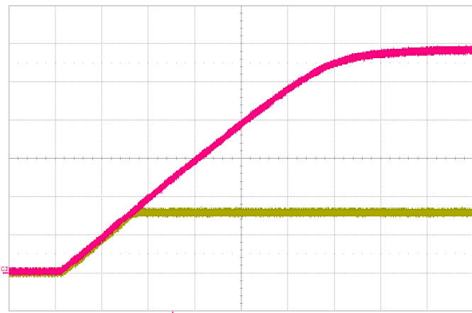
Start-up V_{IN}=12V , I_O=26A Red: Input Voltage Yellow: Output Voltage
