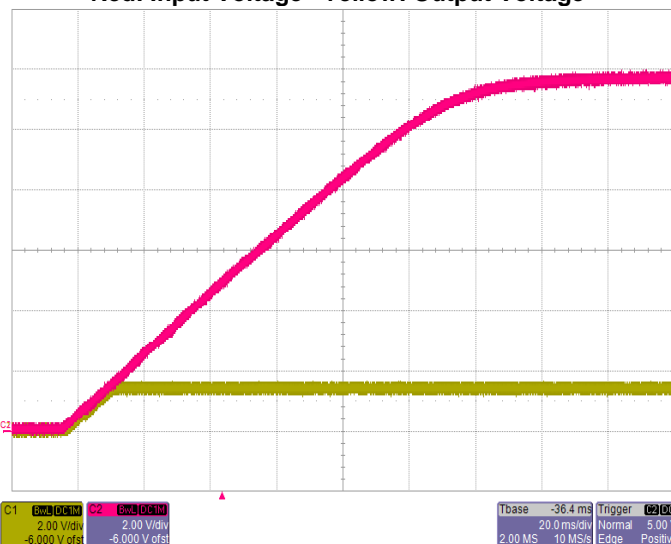
Power Up with EasyTrack™ Control V_{Track}=12.0V , I_O=26A Red: EasyTrack™ Control Voltage Yellow: Output Voltage
