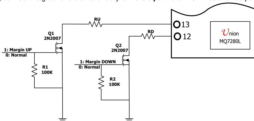
Fig 6 Margin up and Margin down application circuit
