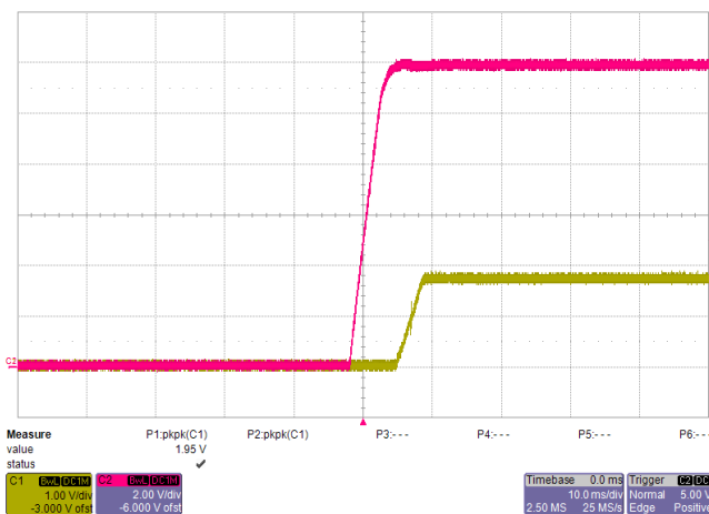
Start-up V_{IN}=12V , I_O=26A Red: Input Voltage Yellow: Output Voltage
