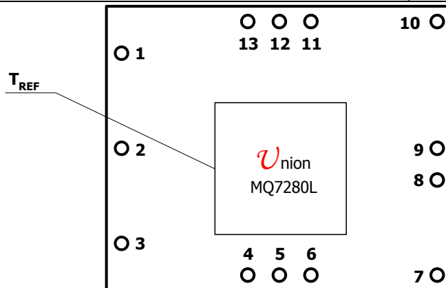
Fig 5, Temperature Reference Point
