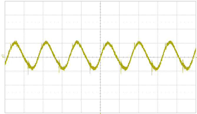
Measure value status P1:pkpk(C1) 49.9 mV C1: 20.0 mV/div, 0.00 mV ofst Timebase: 0.00 µs, Trigger: 2.00 µs/div, Auto, -400 µV, 100 kS, 5.0 GS/s, Edge, Positive
