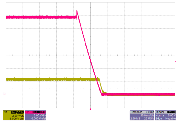
Power Down with EasyTrack™ Control V_{Track}=12.0V , I_O=26A Red: EasyTrack™ Control Voltage Yellow: Output Voltage
