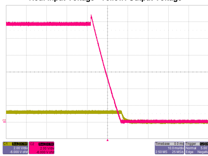
Power Down with EasyTrack™ Control V_{Track}=12.0V , I_O=26A Red: EasyTrack™ Control Voltage Yellow: Output Voltage
