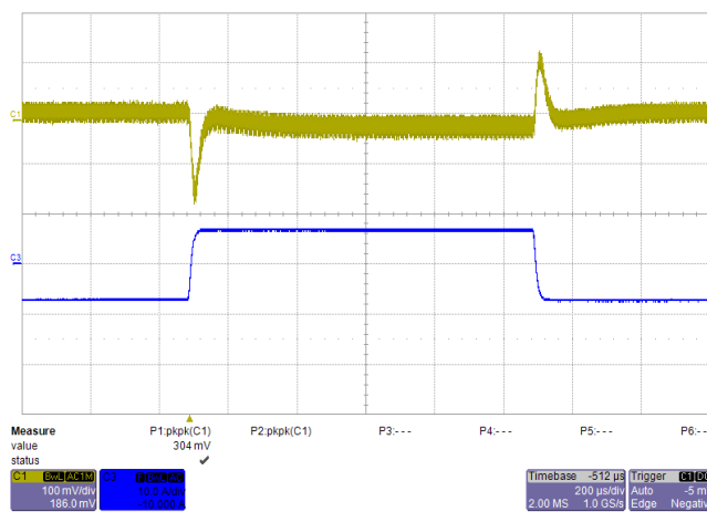
Transient Response V_{IN}=12V , Step from 13A~26A~13A Blue: Output Current Yellow: Output Ripple
