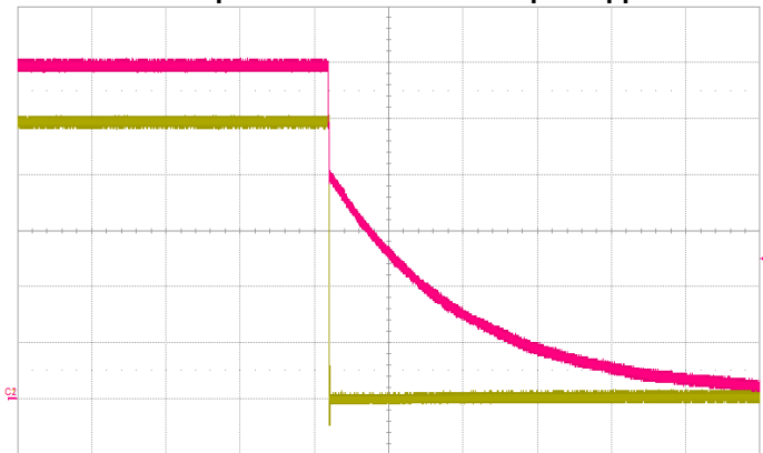
Measure value status P1:pkpk(C1) 5.54 V C1: 1.00 V/div, -3.000 V ofst C2: 6.00 V/div, -6.000 V ofst Timebase: 0.00 s, Trigger: 500 ms/div, Normal, 5.00 V, 2.50 MS, 25 MS/s, Edge, Negative
