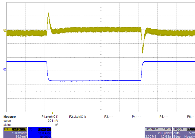
Transient Response V_{IN}=12V , Step from 13A~26A~13A Blue: Output Current Yellow: Output Ripple
