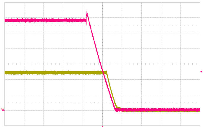
C1: 2.00 V/div, -6.000 V ofst C2: 2.00 V/div, -6.000 V ofst Timebase: 0.0 ms, Trigger: 10.0 ms/div, Normal, 5.00 V, 2.50 MS, 25 MS/s, Edge, Negative
