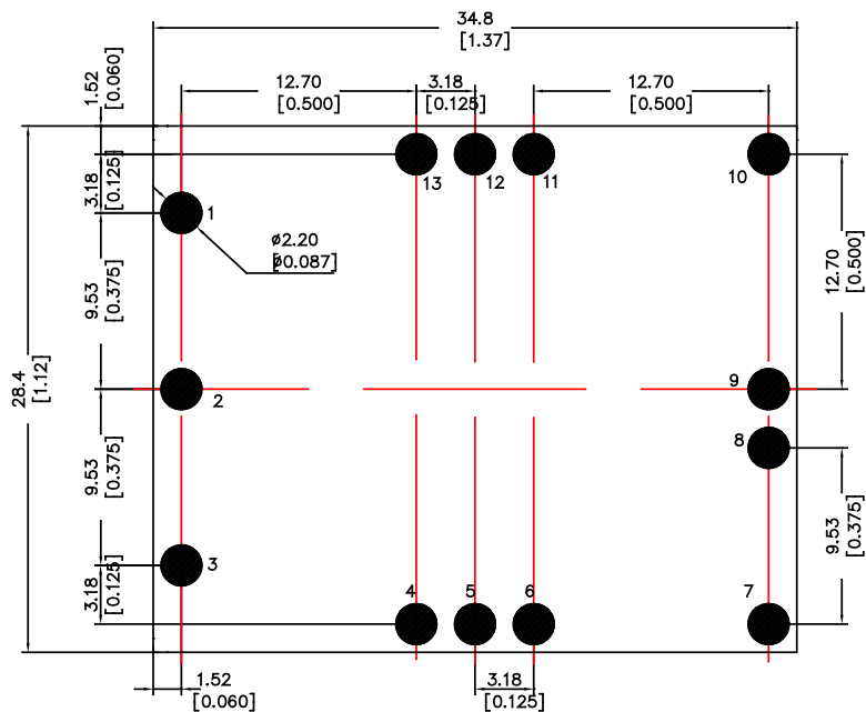
Component-side footprint
