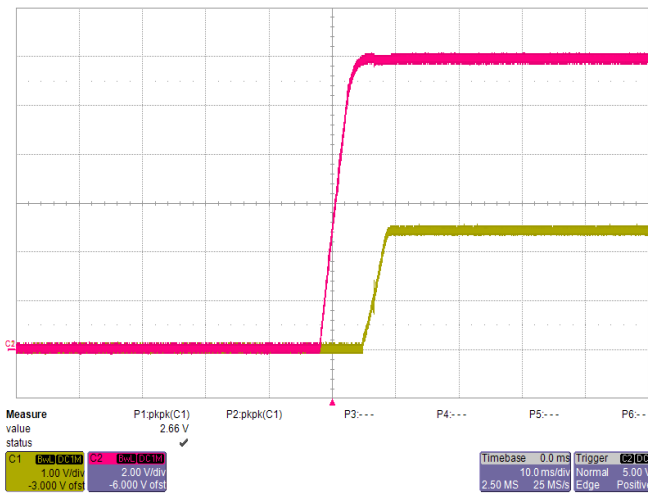
Start-up V_{IN}=12V , I_O=26A Red: Input Voltage Yellow: Output Voltage
