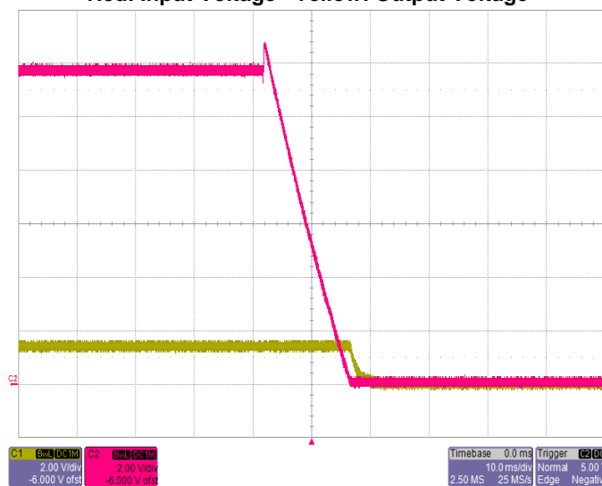
Power Down with EasyTrack™ Control V_{Track}=12.0V , I_O=26A Red: EasyTrack™ Control Voltage Yellow: Output Voltage
