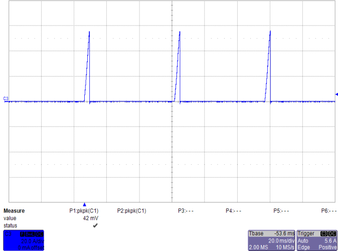
Short-Circuit Output V_{IN}=12V
