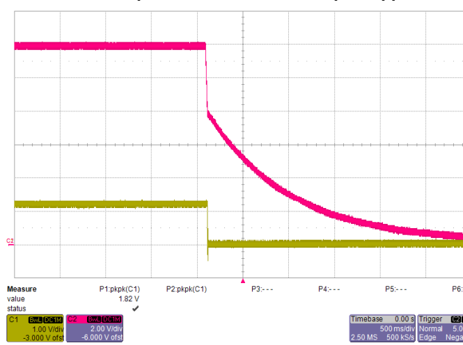
Shut-down V_{IN}=12V , I_O=26A Red: Input Voltage Yellow: Output Voltage
