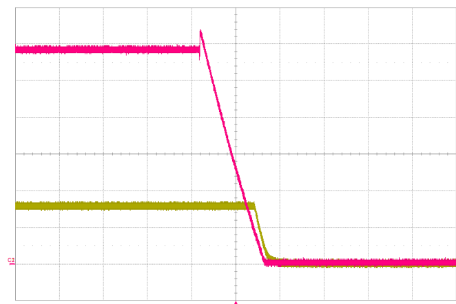
Shut-down V_{IN}=12V , I_O=26A Red: Input Voltage Yellow: Output Voltage
