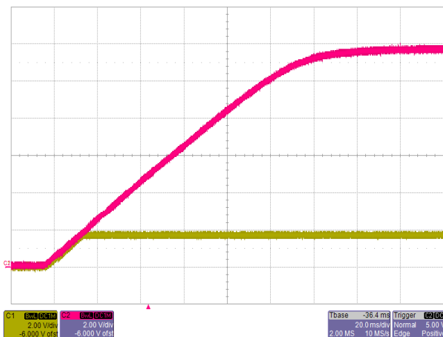
Power Up with EasyTrack™ Control V_{Track}=12.0V , I_O=26A Red: EasyTrack™ Control Voltage Yellow: Output Voltage
