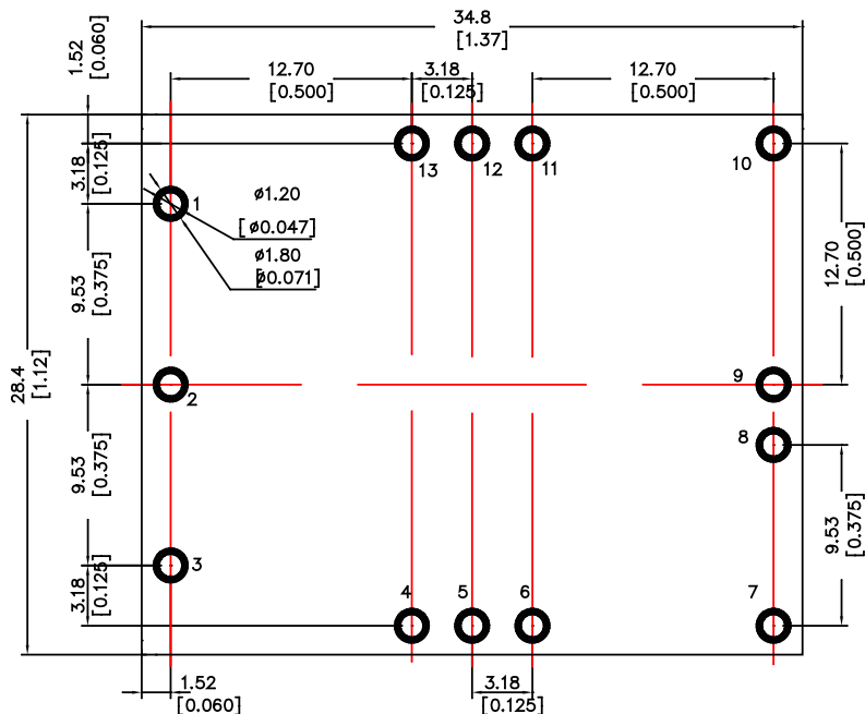
Component-side footprint
