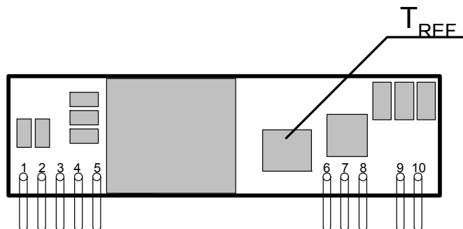
Fig2, Temperature Reference Point
