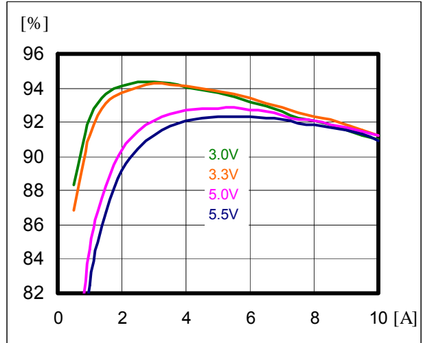
Efficiency
