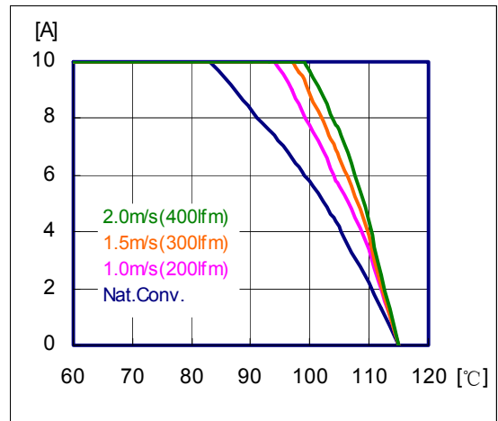
Output Current Derating (Load Current vs. Ambient Temperature ( T_{REF} , See Page 6 )), V_{IN}=3.3V
