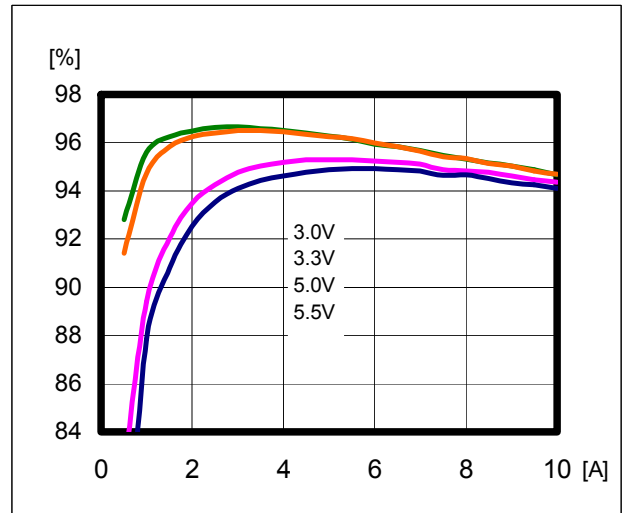
Efficiency
