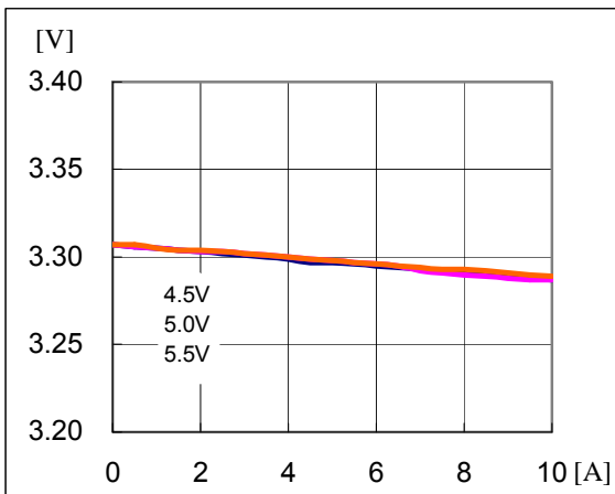
Regulation Output voltage vs. Load Current
