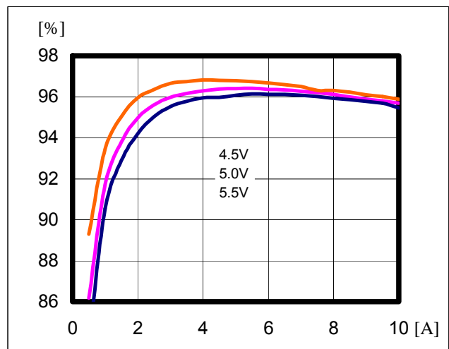
Efficiency
