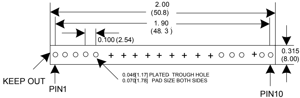
Component-side footprint
