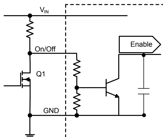
Fig1b. Circuit configuration for using negative logic On/OFF
