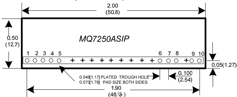
Component-side footprint
