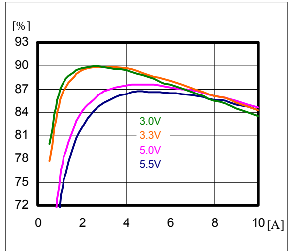
Efficiency
