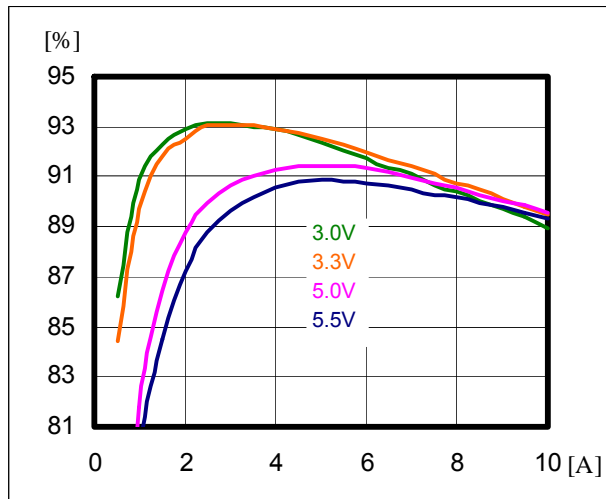
Efficiency
