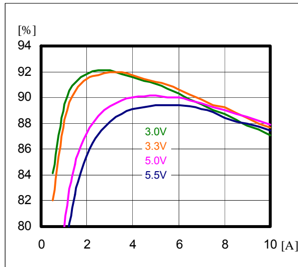
Efficiency
