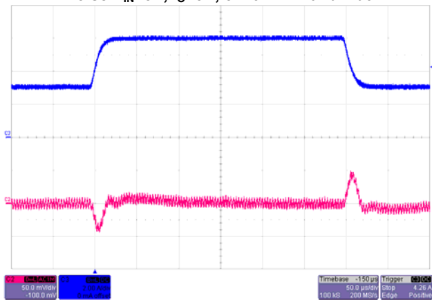
Transient Response V_{IN}=5V , Step from 6A~3A~6A Cin=47µF*4, Cout=47µF*2
