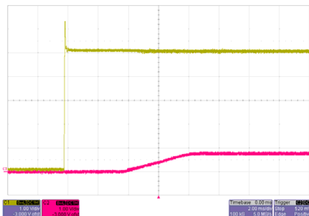
Start-up V_{IN}=5V , I_O=5A
