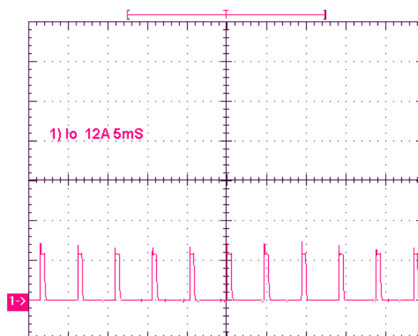
Short-Circuit Output V_{IN}=3.3V
