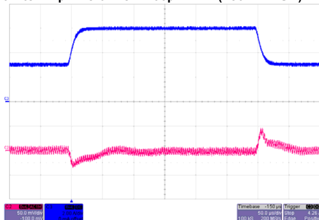
Transient Response V_{IN}=5V , Step from 6A~3A~6A C_{in}=47\mu F*4 , C_{out}=47\mu F*2
