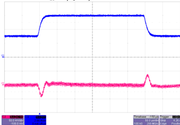
Transient Response V_{IN}=5V , Step from 3A~6A~3A C_{in}=47\mu F \times 4 , C_{out}=47\mu F \times 2
