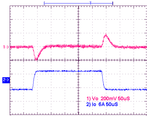
Transient Response V_{IN}=12V , Step from 8A~16A~8A
