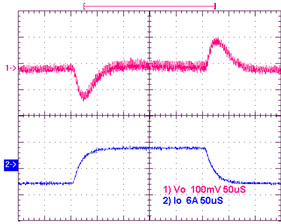
Transient Response V_{IN}=12V , Step from 8A~16A~8A
