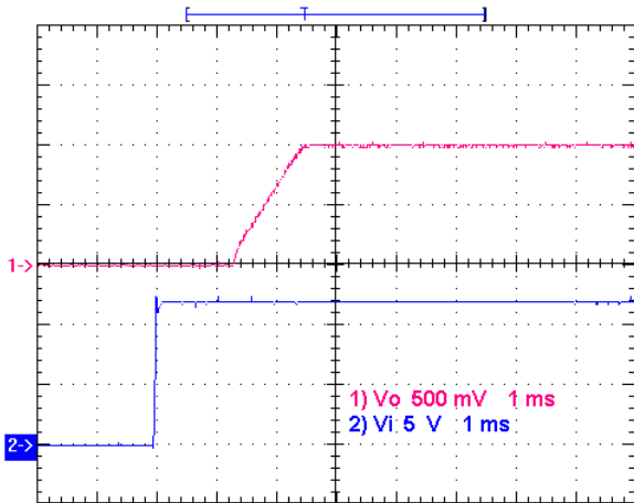
Start-up V_{IN}=12V , I_o=16A
