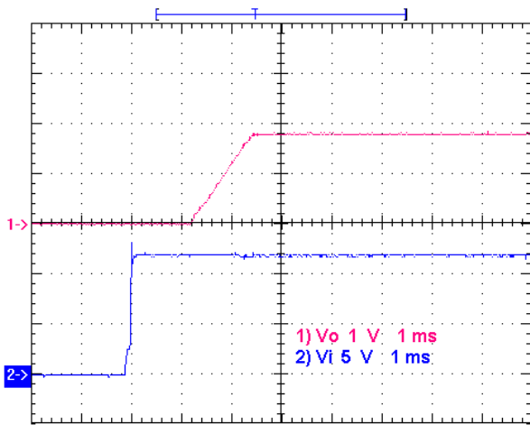
Start-up V_{IN}=12V , I_O=16A
