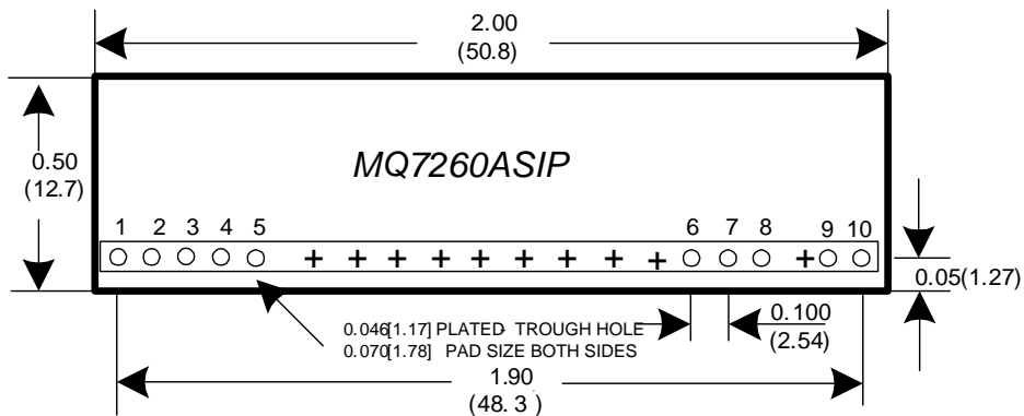
Component-side footprint
