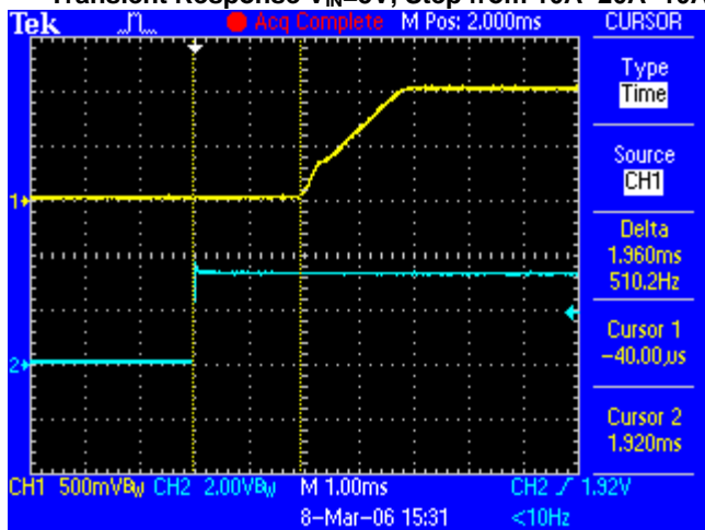
Start-up V_{IN}=3.3V , I_O=15.6A (resistive load)
