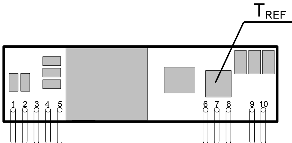
Fig2, Temperature Reference Point
