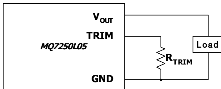
Fig6. Circuit configuration for programming output voltage using external resistor
