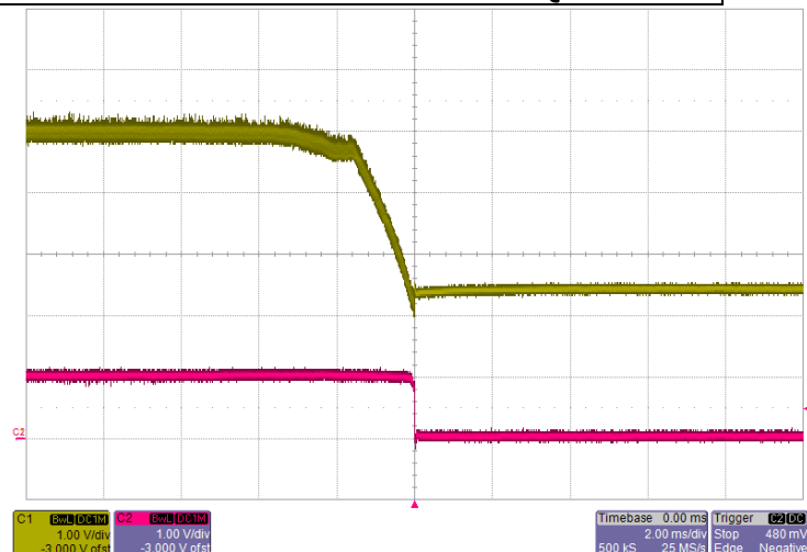
Start-up V_{IN}=5V , I_O=10A Red: Input Voltage Yellow: Output Voltage
