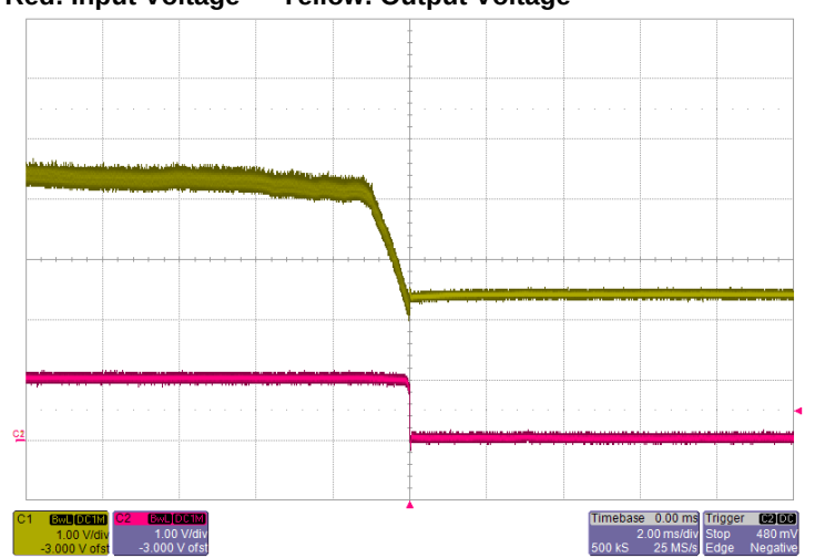
Shut-down V_{IN}=4.5V , I_O=10A Red: Input Voltage Yellow: Output Voltage
