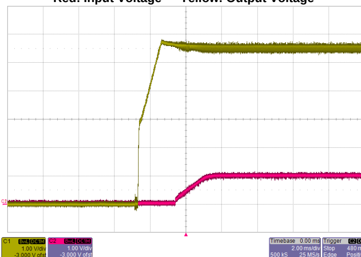
Start-up V_{IN}=5.5V , I_O=10A Red: Input Voltage Yellow: Output Voltage
