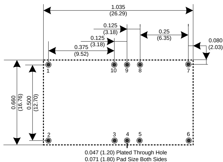
Component-side footprint
