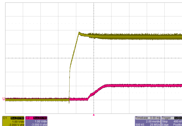
Start-up V_{IN}=4.5V , I_O=10A Red: Input Voltage Yellow: Output Voltage
