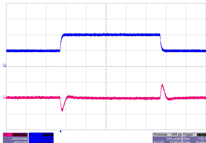
Transient Response V_{IN}=4.5V , Step from 50%~100%~50% Blue: Output Current Yellow: Output Ripple
