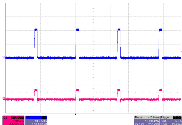
Short-Circuit Output V_{IN}=5.5V
