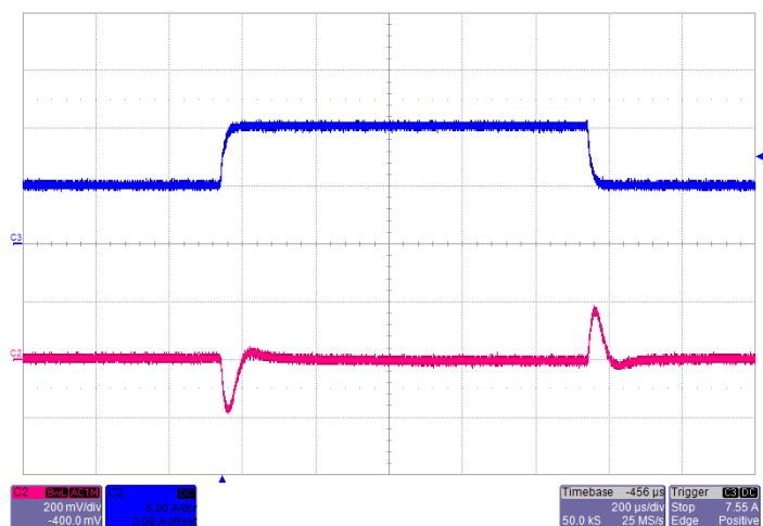
Transient Response V_{IN}=5V , Step from 50%~100%~50% Blue: Output Current Yellow: Output Ripple
