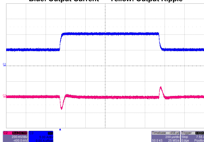
Transient Response V_{IN}=5.5V , Step from 50%~100%~50% Blue: Output Current Yellow: Output Ripple
