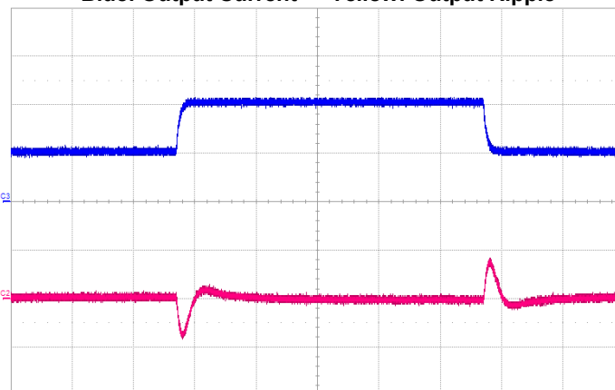
Transient Response V_{IN}=4.5V , Step from 50%~100%~50% Blue: Output Current Yellow: Output Ripple
