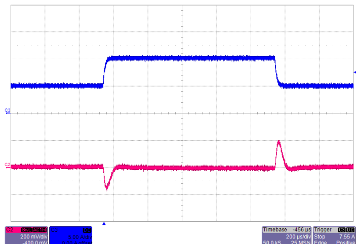
Transient Response V_{IN}=5V , Step from 50%~100%~50% Blue: Output Current Yellow: Output Ripple
