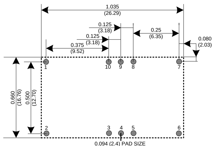
Component-side footprint
