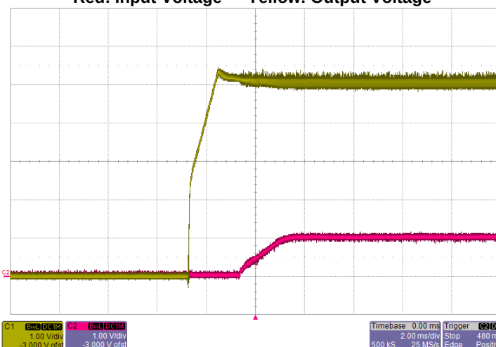
Shut-down V_{IN}=5V , I_O=10A Red: Input Voltage Yellow: Output Voltage
