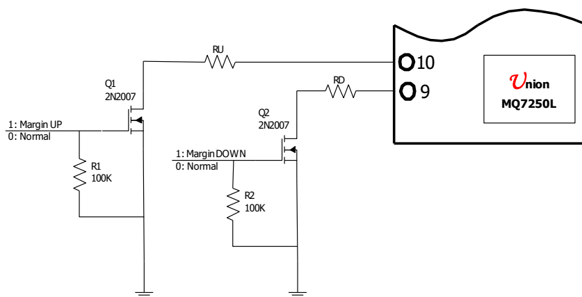
Fig4 Margin up and Margin down application circuit
