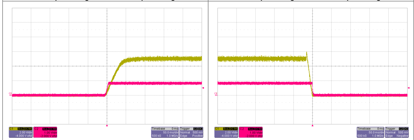
Power Up with EasyTrack™ Control V_{Track}=5.0V , I_O=22A Yellow: EasyTrack™ Control Voltage Red: Output Voltage
