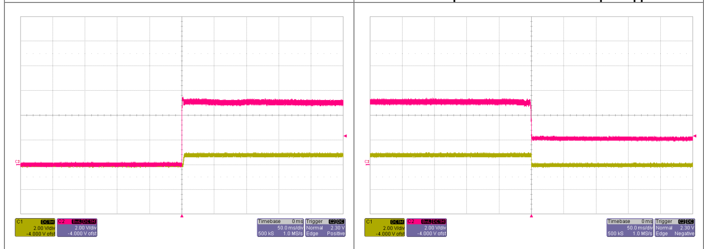
Start-up V_{IN}=3.3V , I_O=22A Red: Input Voltage Yellow: Output Voltage
