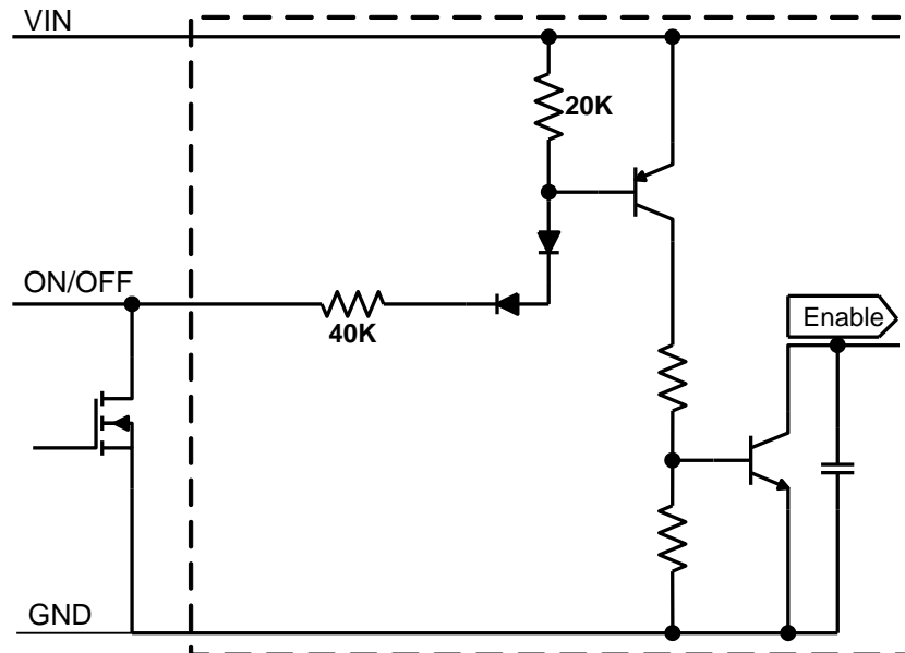
Fig5, Remote ON/OFF Implementation with Open Collector/Drain transistor for positive logic control
