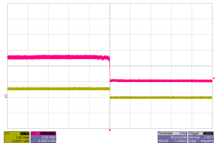
Shut-down V_{IN}=3.3V , I_O=22A Red: Input Voltage Yellow: Output Voltage
