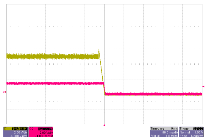
Power Down with EasyTrack™ Control V_{Track}=5.0V , I_O=22A Yellow: EasyTrack™ Control Voltage Red: Output Voltage
