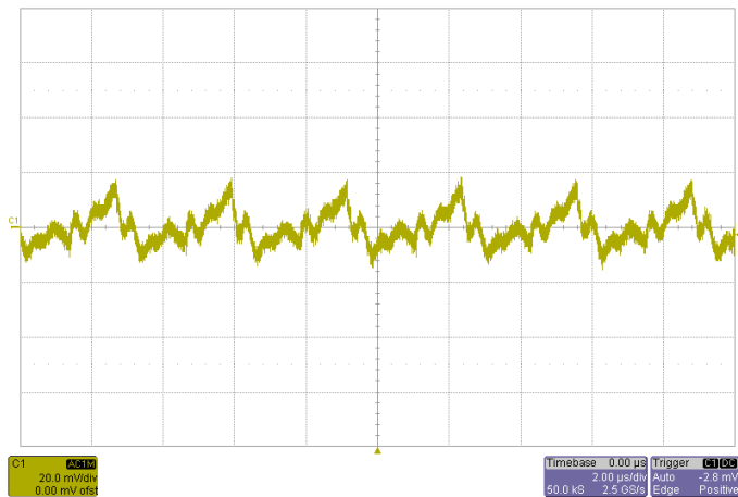
Noise V_{IN}=3.3V , I_O=22A , 5~20MHz Bandwidth
