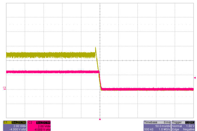
Power Down with Auto-Track Control V_{Track}=5.0V , I_O=22A Red: EasyTrack™ Control Voltage Yellow: Output Voltage
