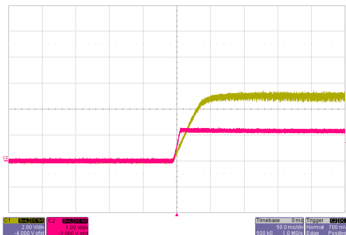
Power Up with EasyTrack™ Control V_{Track}=5.0V , I_O=22A Yellow: EasyTrack™ Control Voltage Red: Output Voltage
