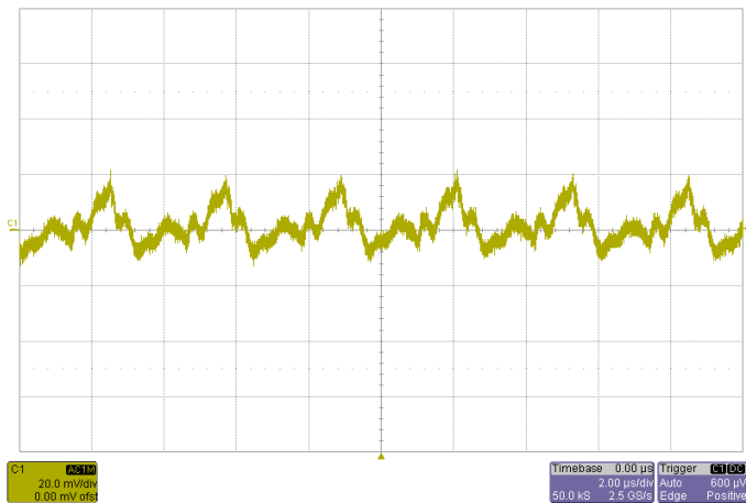
Noise V_{IN}=3.3V , I_O=22A , 5~20MHz Bandwidth
