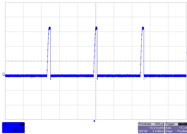
Short-Circuit Output V_{IN}=3.3V
