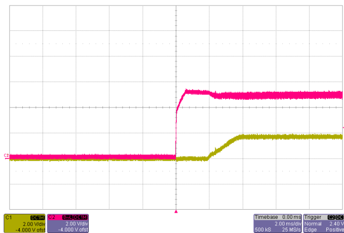
Start-up V_{IN}=3.3V , I_O=22A Red: Input Voltage Yellow: Output Voltage
