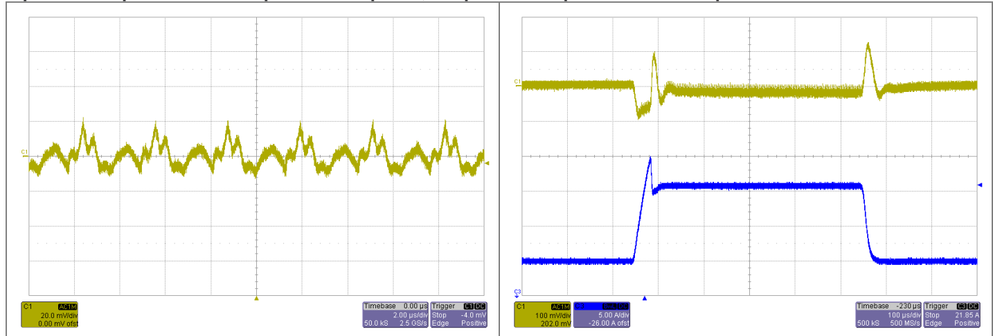
Transient Response V_{IN}=3.3V , Step from 11A~22A~11A Blue: Output Current Yellow: Output Ripple
