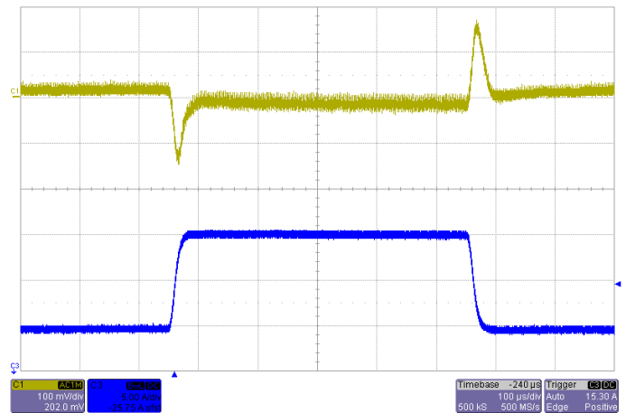
Transient Response V_{IN}=3.3V , Step from 11A~22A~11A Blue: Output Current Yellow: Output Ripple
