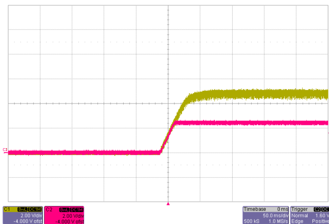
Power Up with Auto-Track Control V_{Track}=5.0V , I_O=22A Red: EasyTrack™ Control Voltage Yellow: Output Voltage
