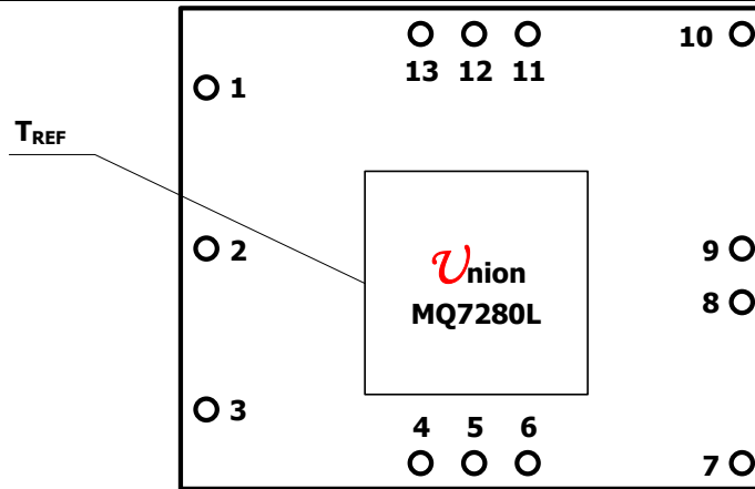
Fig 5, Temperature Reference Point
