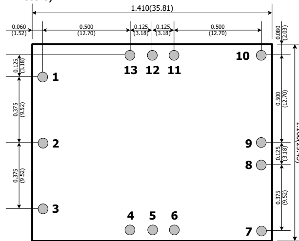
Component-side footprint
