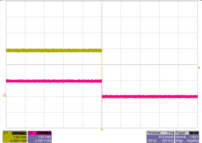
Power Down with ON/OFF Control
