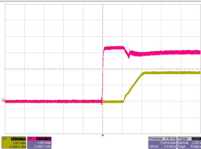
Start-up V_{IN}=3.3V , I_O=30A Red: Input Voltage Yellow: Output Voltage
