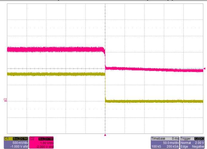
Shut-down V_{IN}=3.3V , I_O=30A Red: Input Voltage Yellow: Output Voltage
