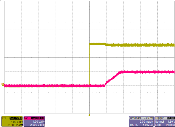
Power Up with ON/OFF Control
