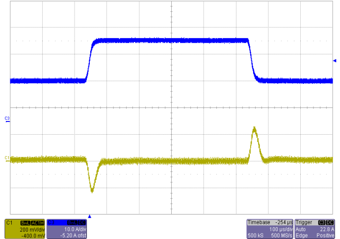
Transient Response V_{IN}=3.3V , Step from 15A~30A~15A Blue: Output Current Yellow: Output Ripple
