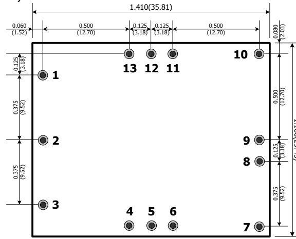
Component-side footprint
