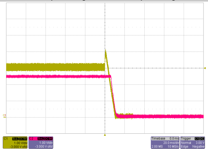
Power Down with Auto-Track Control V_{Track}=5.0V , I_O=30A Yellow: EasyTrack™ Control Voltage Red: Output Voltage
