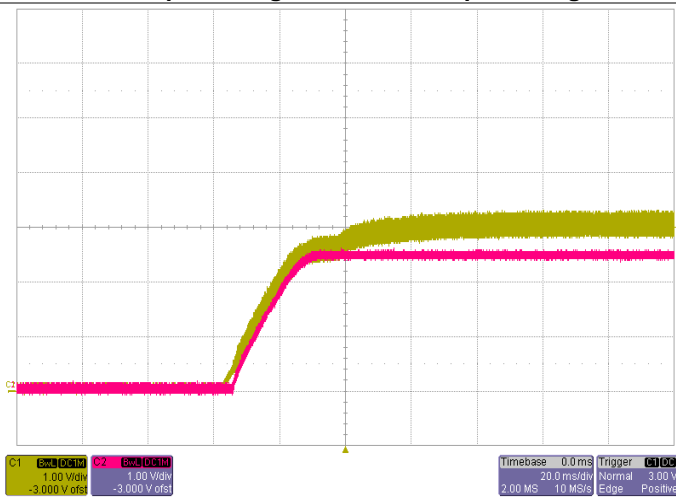
Power Up with Auto-Track Control V_{Track}=5.0V , I_O=30A Yellow: EasyTrack™ Control Voltage Red: Output Voltage
