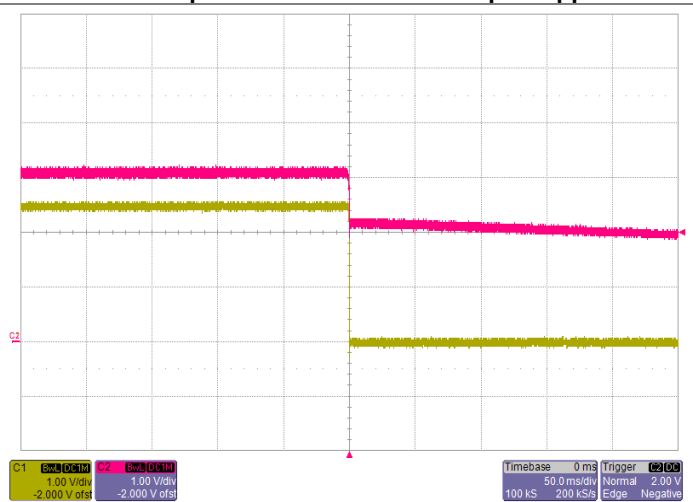
Shut-down V_{IN}=3.3V , I_O=30A Red: Input Voltage Yellow: Output Voltage
