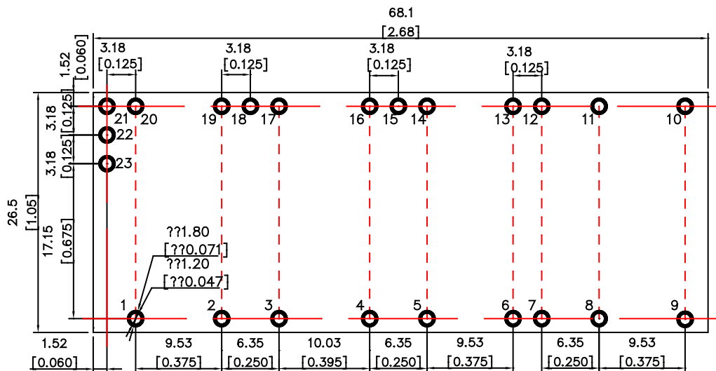
Component-side footprint
