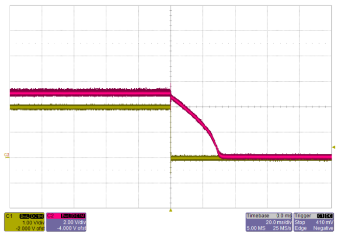
Shut-down V_{IN}=12V , I_O=100A Red: Input Voltage Yellow: Output Voltage
