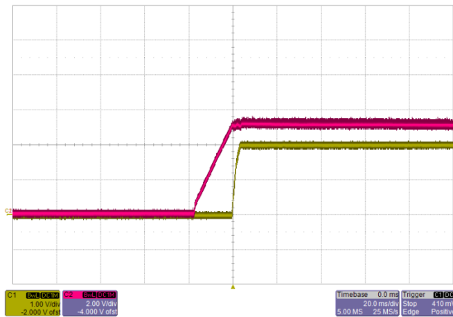
Start-up V_{IN}=12V , I_O=100A Red: Input Voltage Yellow: Output Voltage
