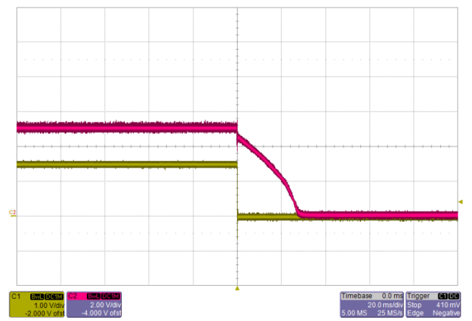
Shut-down V_{IN}=5V , I_O=50A Red: Input Voltage Yellow: Output Voltage
