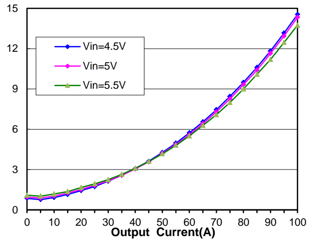
Power Dissipation(W) vs. Load Current(A)
