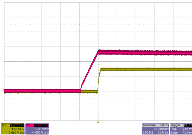
Start-up V_{IN}=5V , I_O=50A Red: Input Voltage Yellow: Output Voltage
