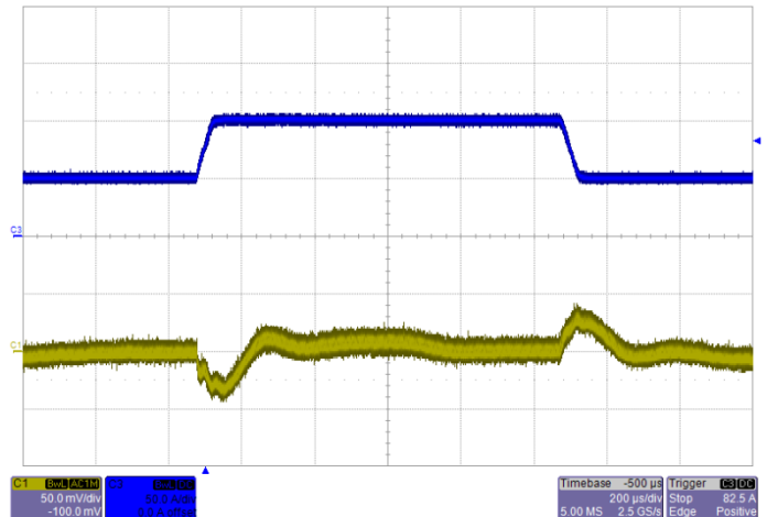
Transient Response V_{IN}=5V , Step from 50A~100A~50A Blue: Output Current Yellow: Output Ripple
