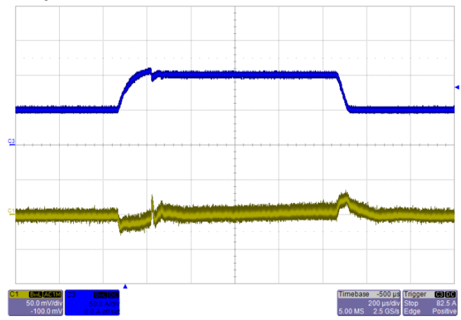
Transient Response V_{IN}=12V , Step from 50A~100A~50A Blue: Output Current Yellow: Output Ripple
