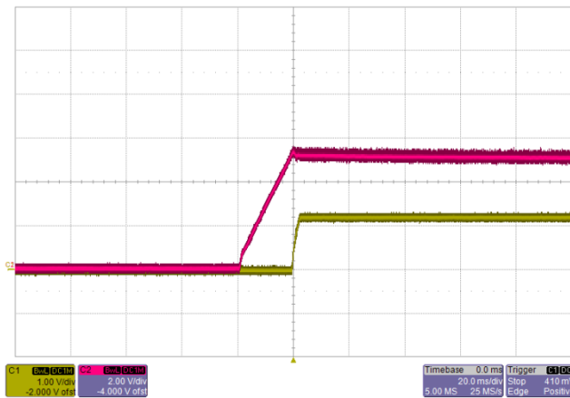
start-up V_{IN}=5V , I_O=100A Red: Input Voltage Yellow: Output Voltage
