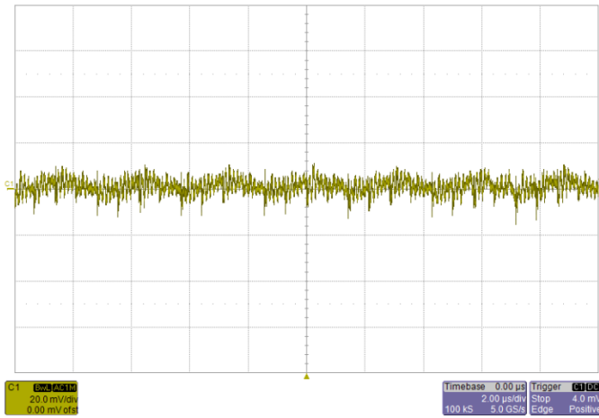
Noise V_{IN}=5V , I_O=100A , 20MHz Bandwidth
