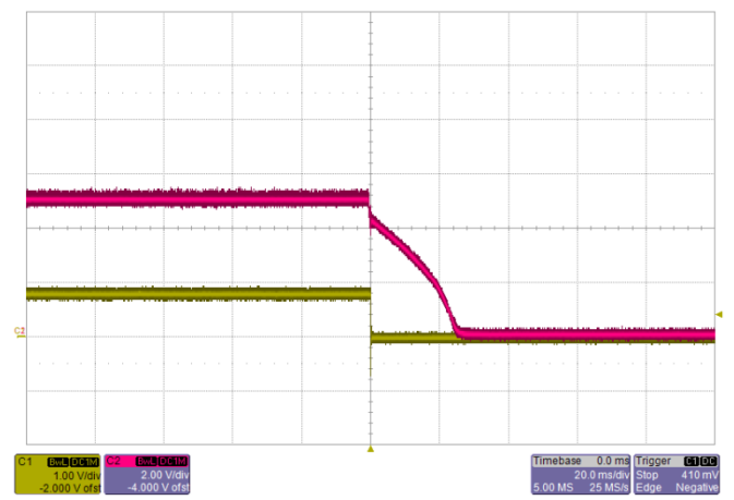
Shut-down V_{IN}=5V , I_O=100A Red: Input Voltage Yellow: Output Voltage
