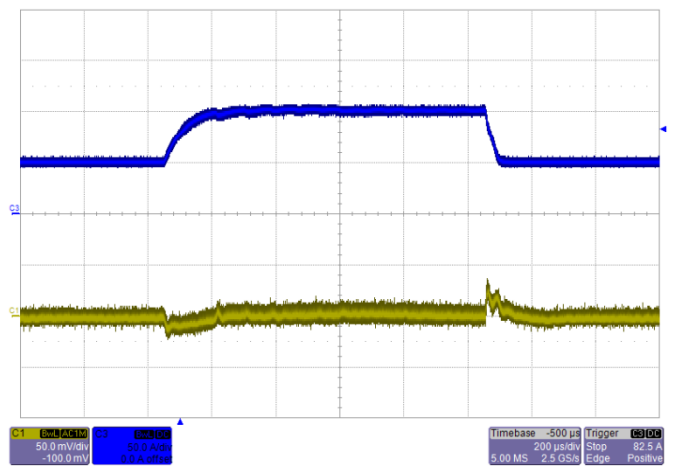
Transient Response V_{IN}=5V , Step from 50A~100A~50A Blue: Output Current Yellow: Output Ripple
