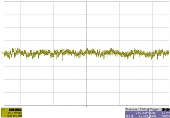
Noise V_{IN}=5V , I_O=100A , 20MHz Bandwidth
