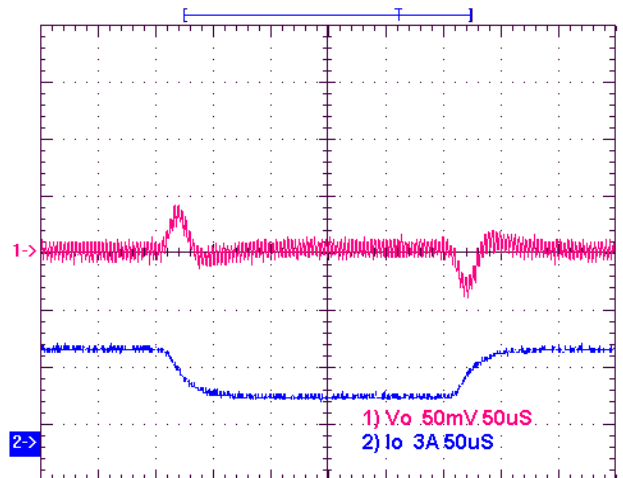
Transient Response V_{IN}=12V , Step from 2.5A~5A~2.5A
