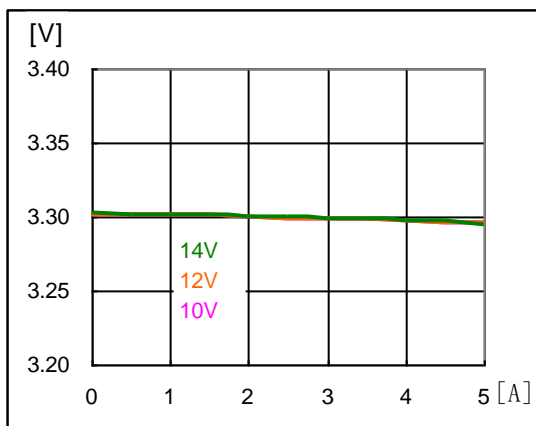
Regulation Output voltage vs. Load Current
