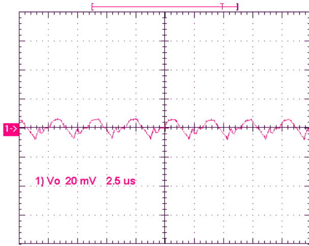
Noise V_{IN}=12V, I_O=5A, 5\sim 20MHz Bandwidth
