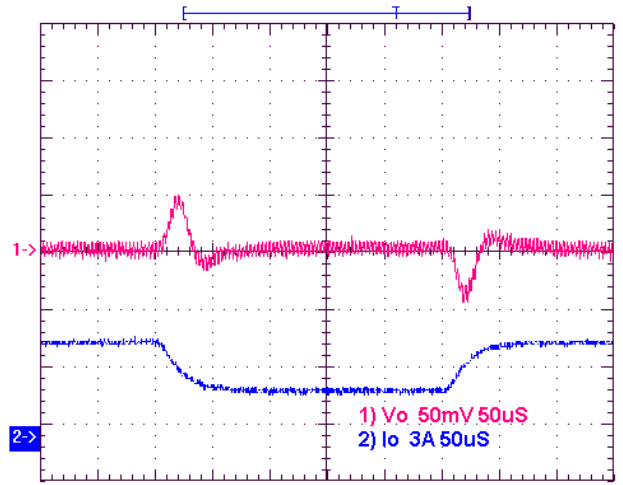
Transient Response V_{IN}=12V, \text{Step from } 2.5A\sim 5A\sim 2.5A
