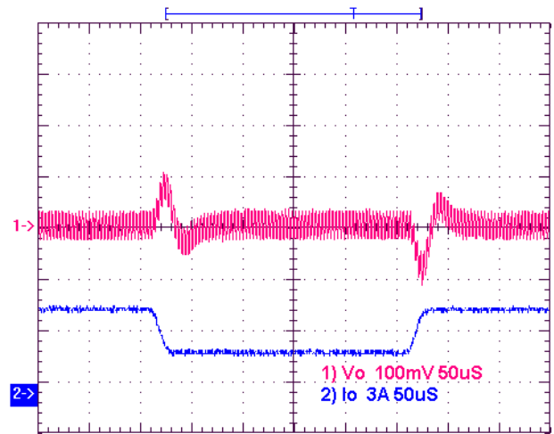
Transient Response V_{IN}=12V , Step from 2.5A~5A~2.5A
