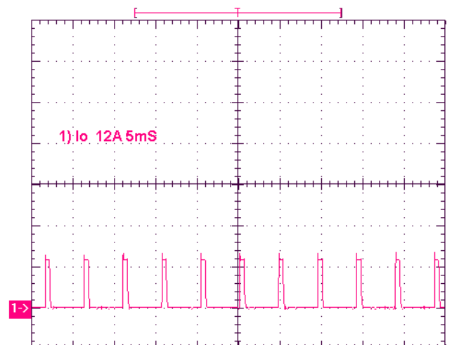
Short-Circuit Output V_{IN}=3.3V
