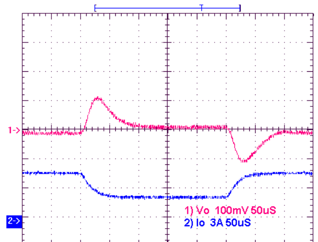
Transient Response V_{IN}=3.3V , Step from 5A~2.5A~5A
