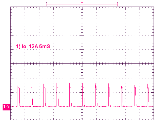
Short-Circuit Output V_{IN}=5V
