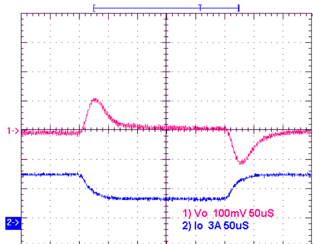
Transient Response V_{IN}=3.3V , Step from 5A~2.5A~5A
