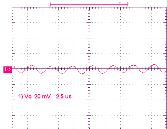
Noise V_{IN}=3.3V , I_O=5A , 5~20MHz Bandwidth
