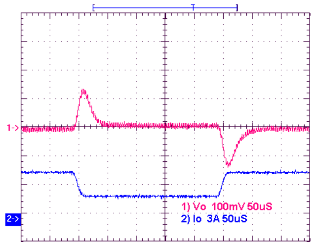
Transient Response V_{IN}=5V , Step from 5A~2.5A~5A
