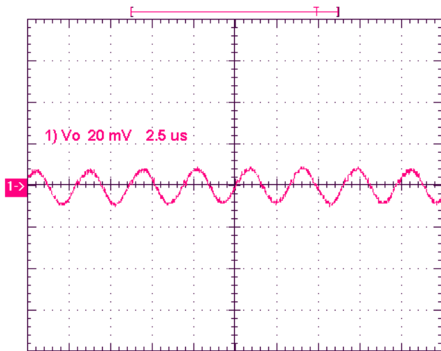
Noise V_{IN}=5V , I_O=5A , 5~20MHz Bandwidth
