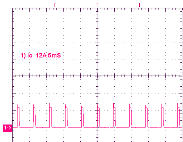
Short-Circuit Output V_{IN}=3.3V
